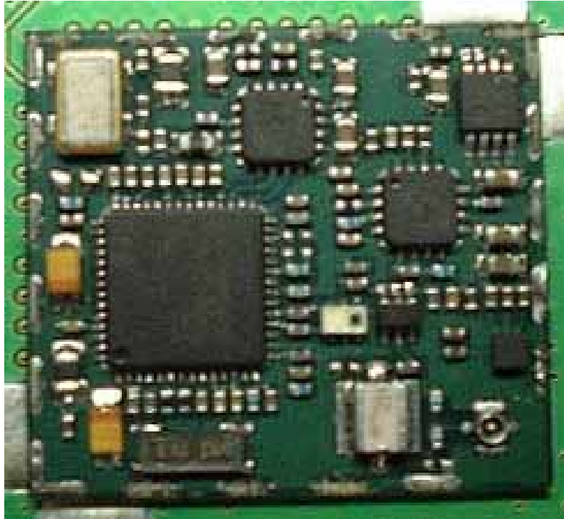
Sychip WLAN Module Top View without shield
