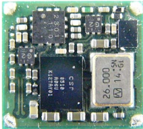
Bluetooth Module Top View
