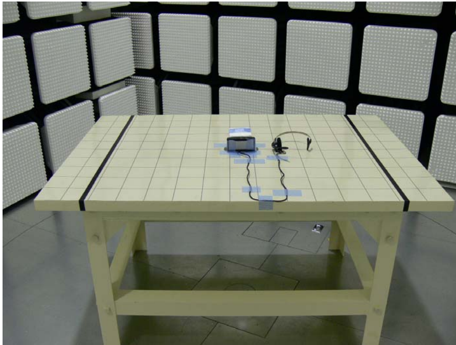
Photograph 2: Set-up for Radiated Emission, EUT Configuration, X axis
