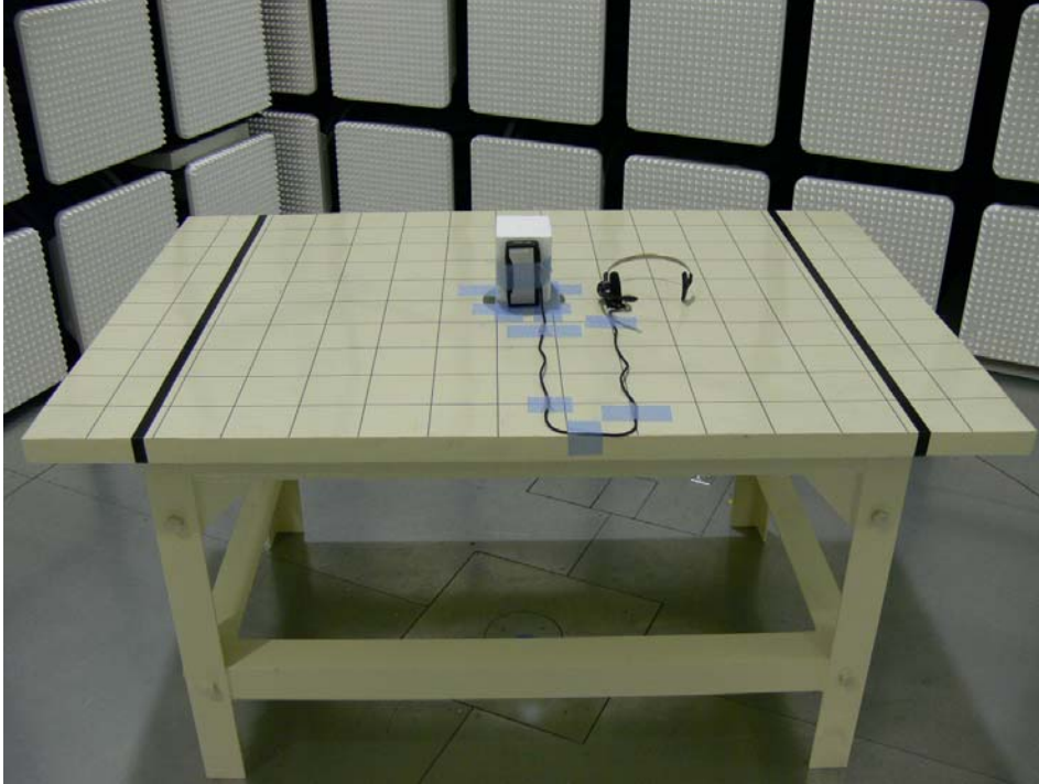
Photograph 1: Set-up for Radiated Emission, EUT Configuration, Y axis
