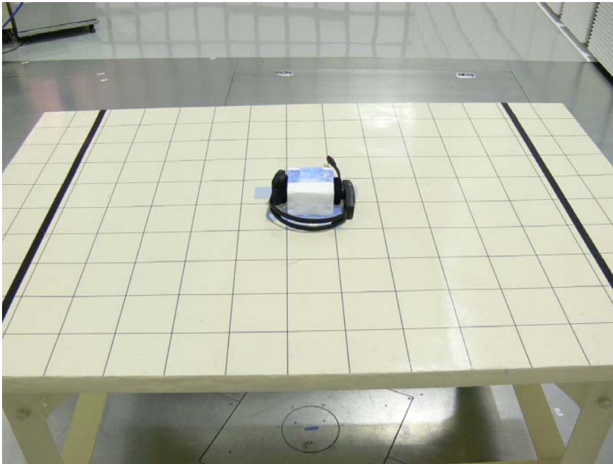
Photograph 2: Set-up for Radiated Emission, EUT Configuration, Y axis
