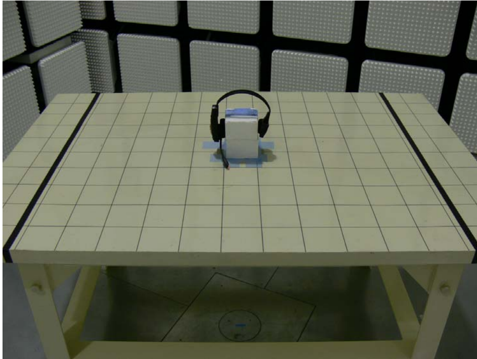
Photograph 1: Set-up for Radiated Emission, EUT Configuration, X axis
