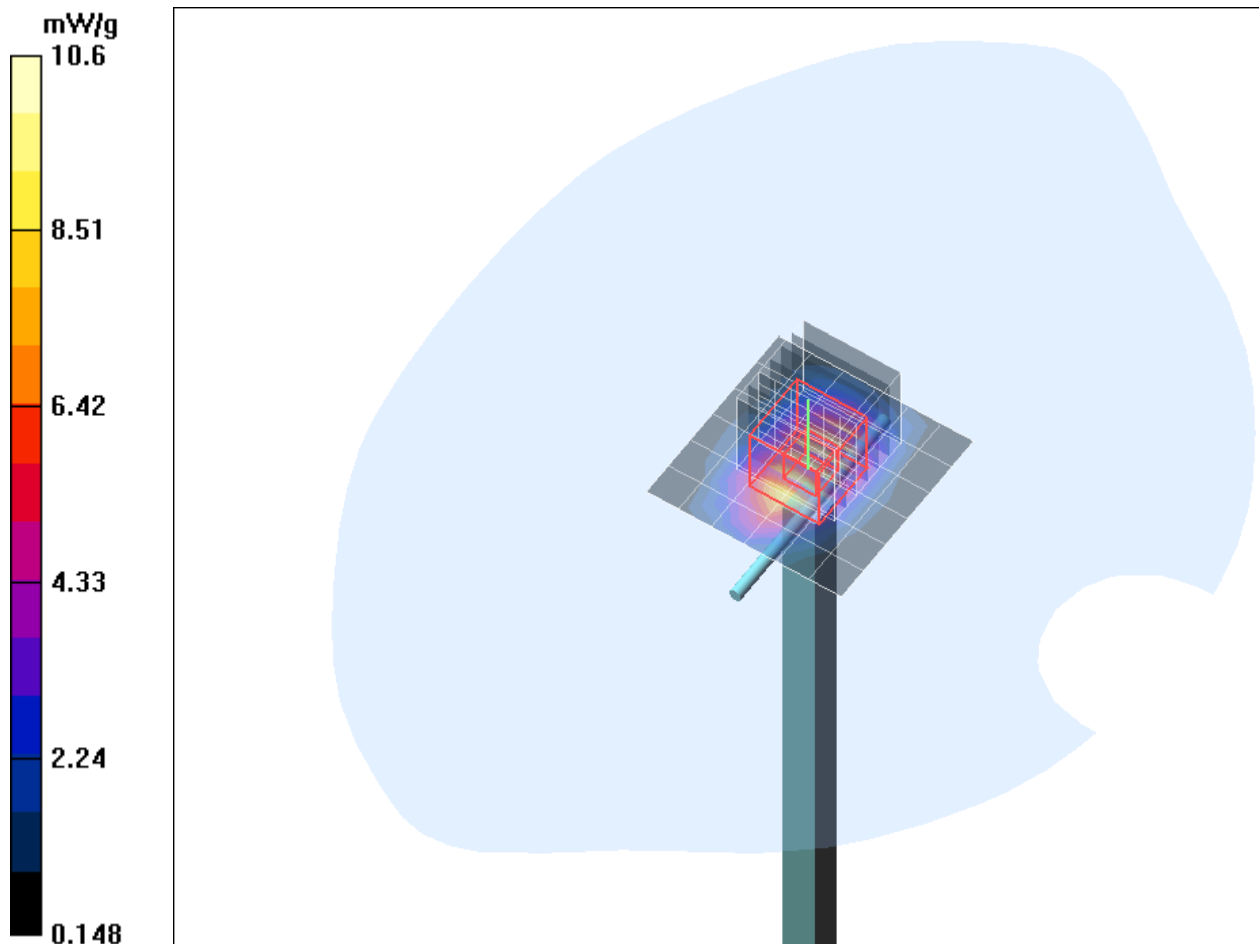
Fig. 5: Validation measurement 1900 MHz Body.
