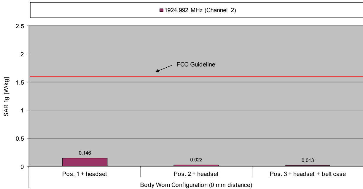
Fig. 4: The reported SAR values for body worn configuration for the Panasonic WX-CT420 in combination with the WX-CT427 headset, for the US DECT standard in comparison to the FCC exposure limit.
