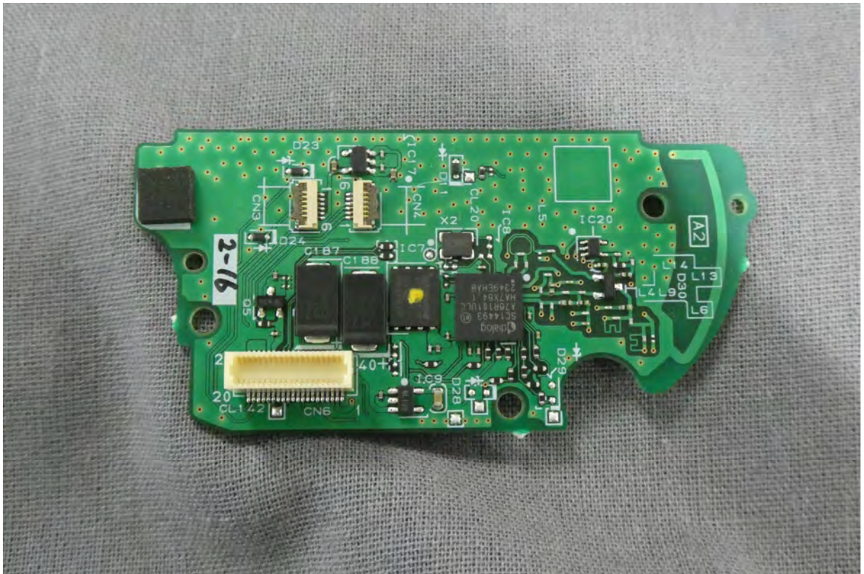
Main Board (including RF block)
