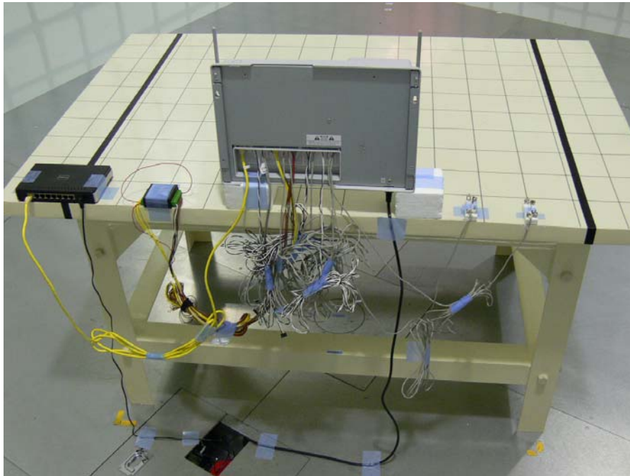
Photograph 4: Set-up for Radiated Emission, EUT Configuration, Back View
