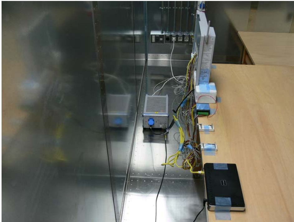
Photograph 2: Set-up for Back View Conducted Testing
