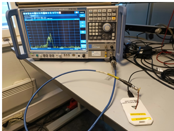
Conducted Test
