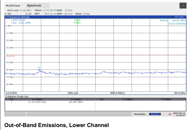
Out-of-Band Emissions, Lower Channel
