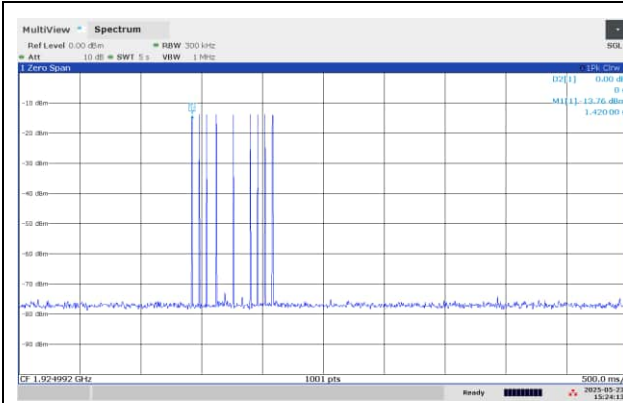
Initial Transmission without Acknowledgements
