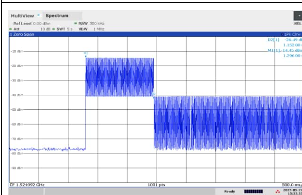
Transmission time after loss of Acknowledgements
