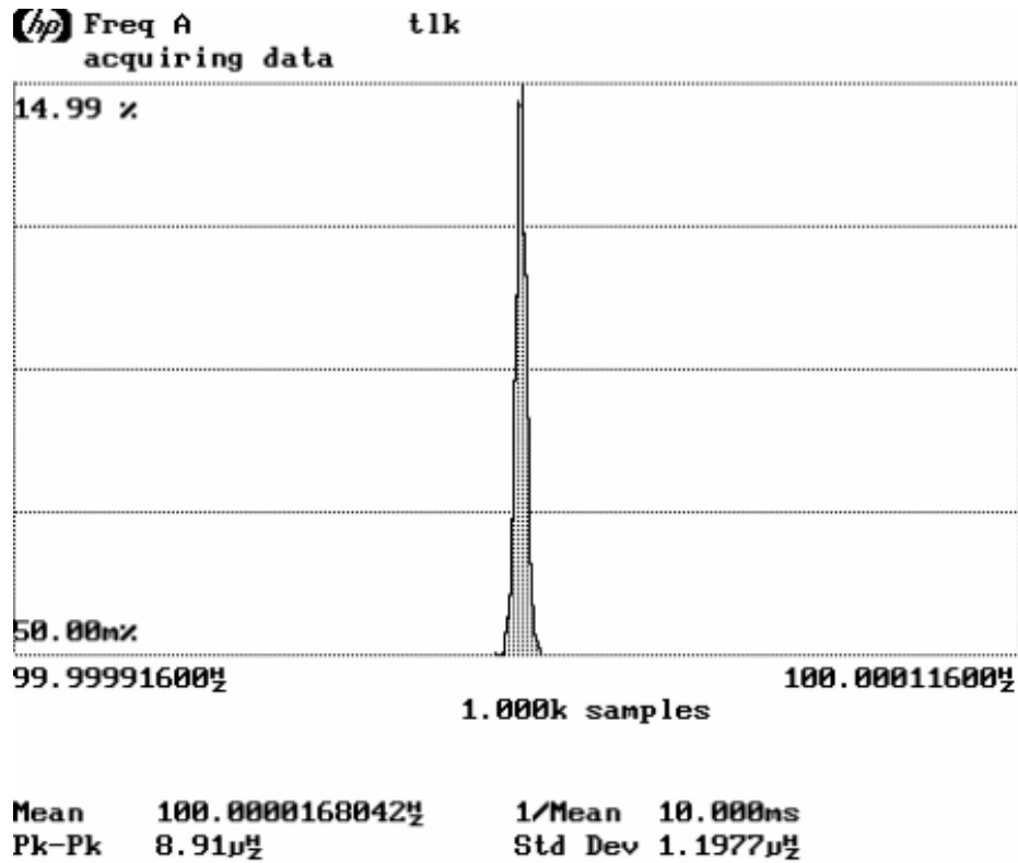
Frame Repetition Stability, Gated over 100 Frames
