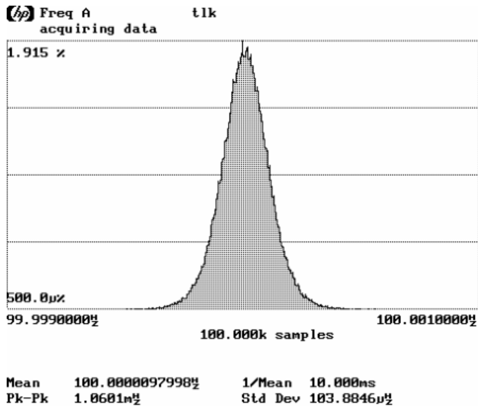
Frame Period and Jitter
