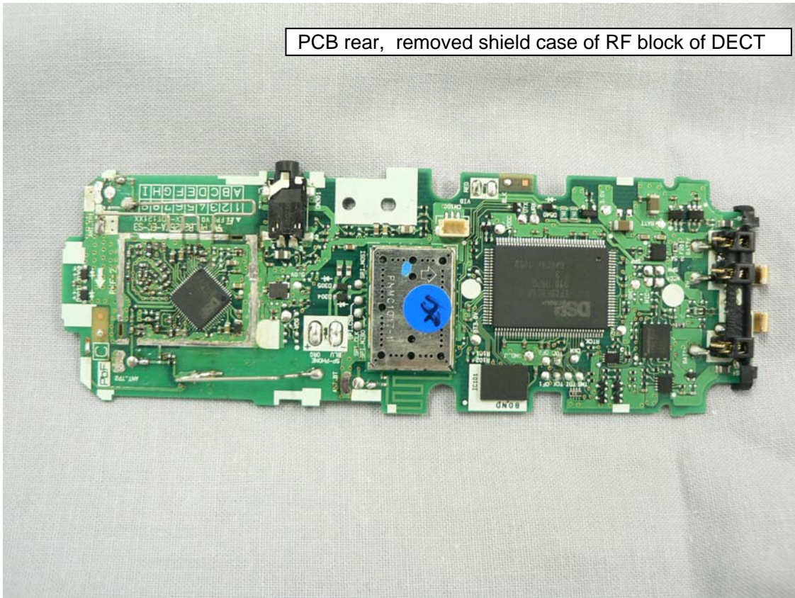
RF block under the shield case of DECT
