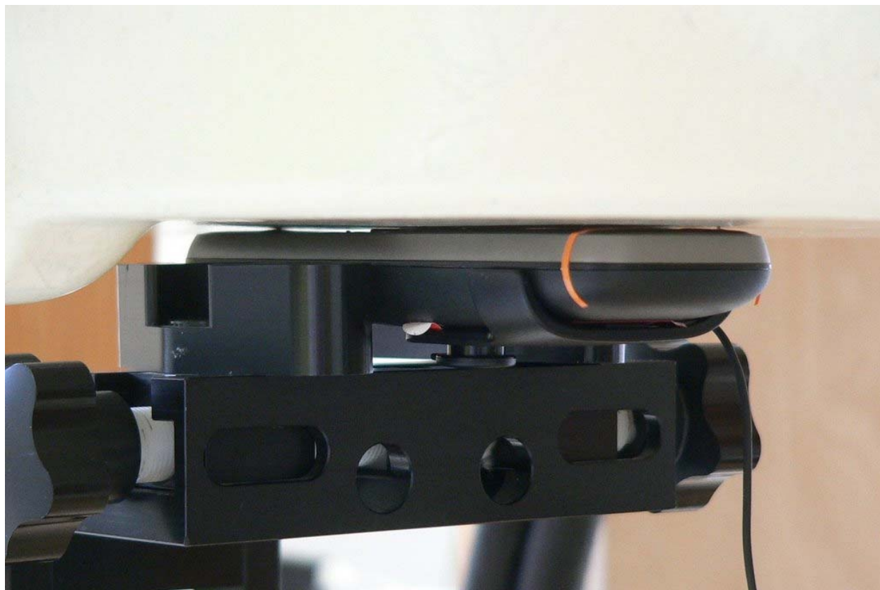
Fig. 8: Body worn configuration for KX-UDT121, position 1, display towards the phantom, headset attached, 0 mm distance.
