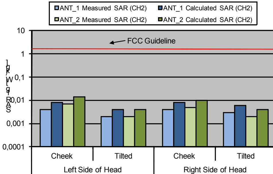
Fig. 8: The measured head phantom SAR values for the Panasonic KX-UDT121, antenna 1 and 2 for the US DECT standard in comparison to the FCC exposure limit.
