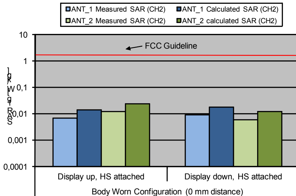
Fig. 9: The measured SAR values in body worn configuration for the Panasonic KX-UDT121, antenna 1 and 2 for the US DECT standard in comparison to the FCC exposure limit.
