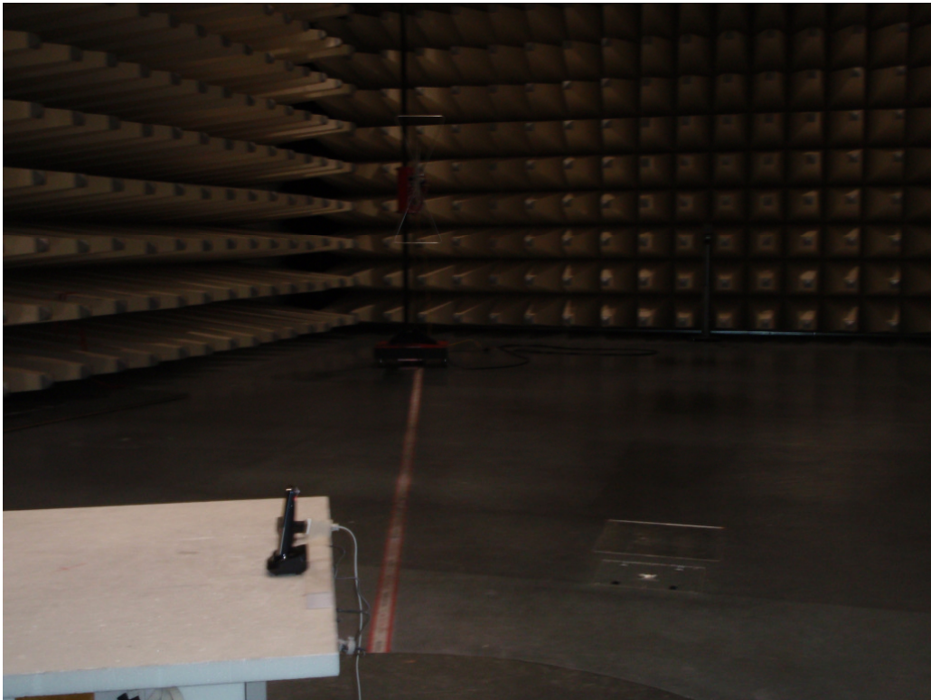
Photo 2: Radiated Emission
