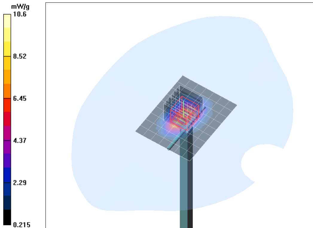
Fig. 9: Validation measurement 1900 MHz Body (March 03, 2016), coarse grid.
