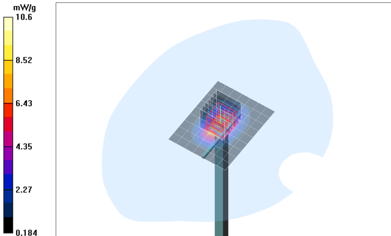
Fig. 8: Validation measurement 1900 MHz Head (February 29, 2016), coarse grid.
