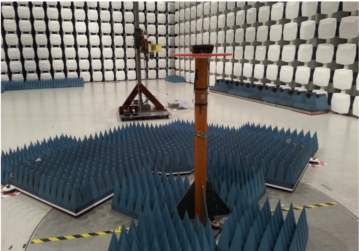
Bluetooth Radiated Emissions Test, 1 - 8.5 GHz
