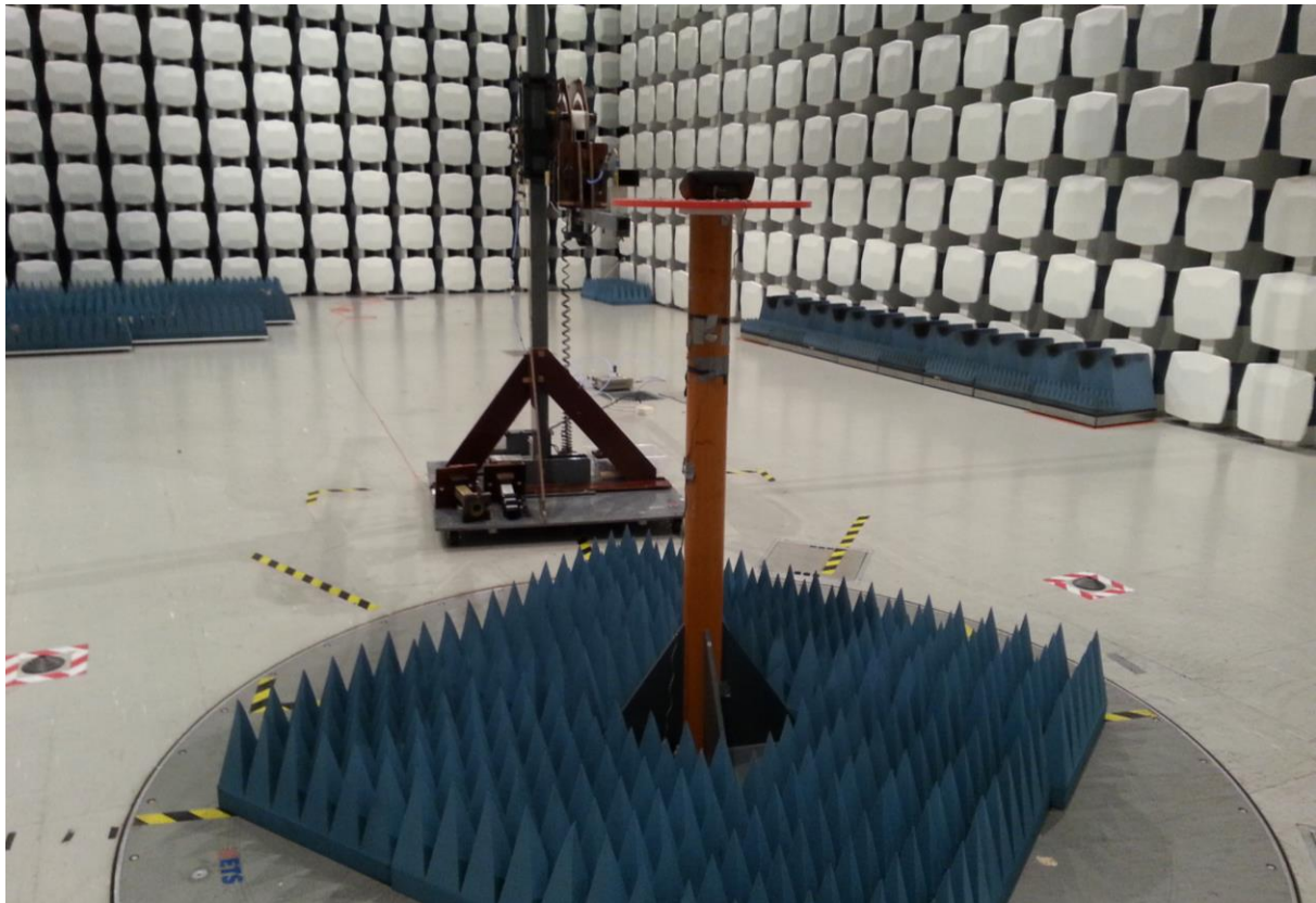
Bluetooth Radiated Emissions Test, 8.5 - 18 GHz
