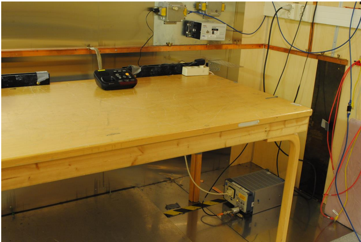
Bluetooth Power line Conducted Emissions Test
