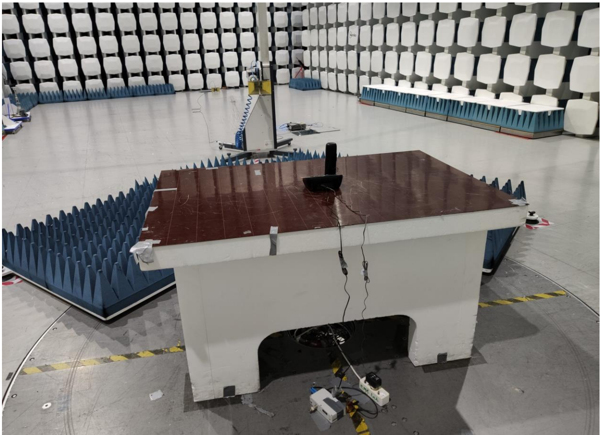
Part 15B Radiated Emissions, 1 GHz – 6 GHz
