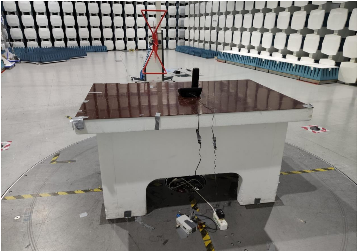
Part 15B Radiated Emissions, 30 - 1000 MHz
