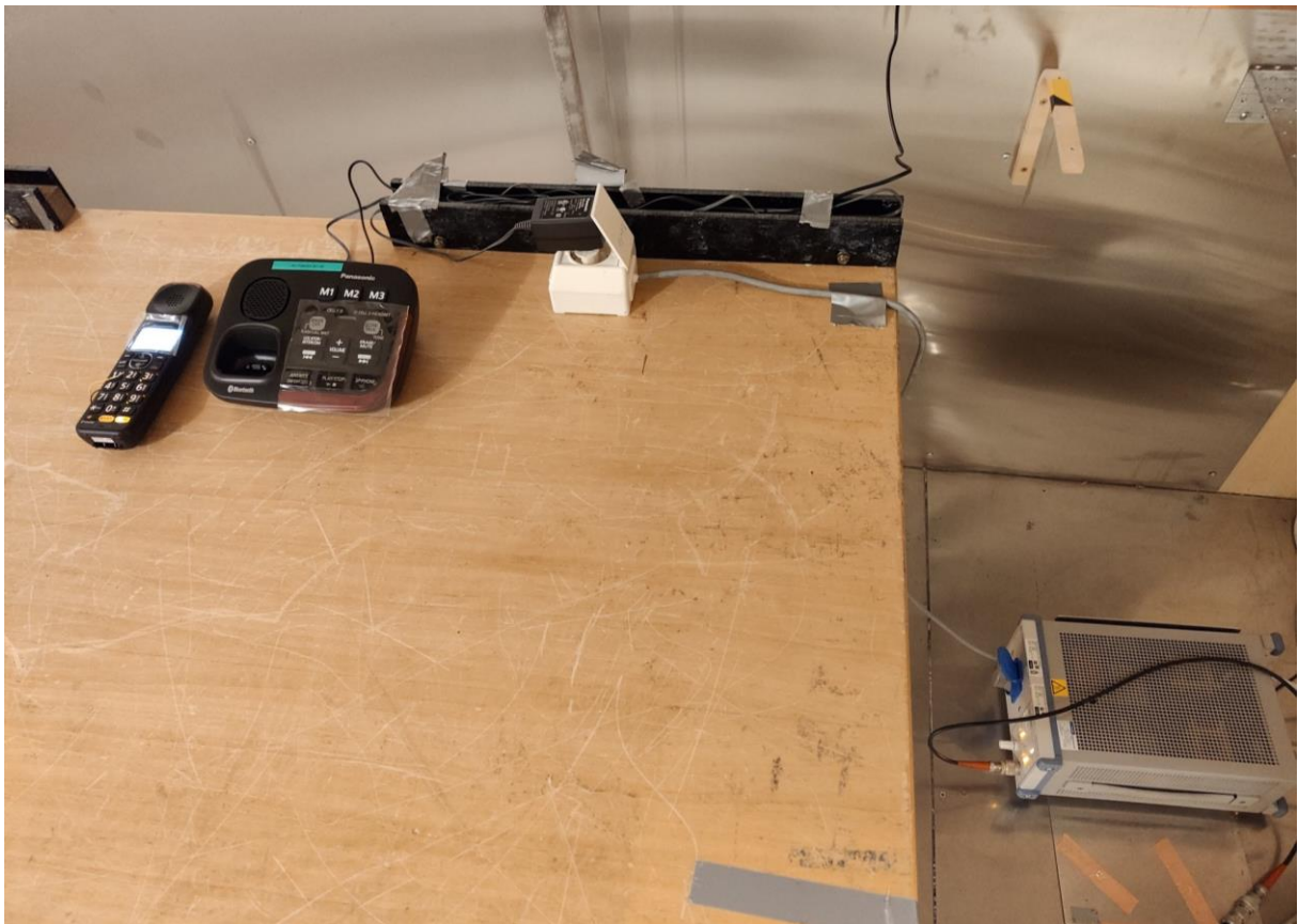
KX-TGM460 Power line Conducted Emissions Test
