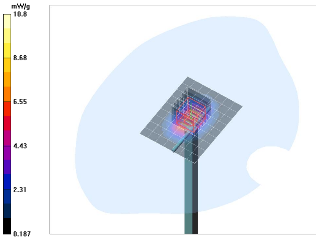
Fig. 8: Validation measurement 1900 MHz Head (November 03, 2015), coarse grid.
