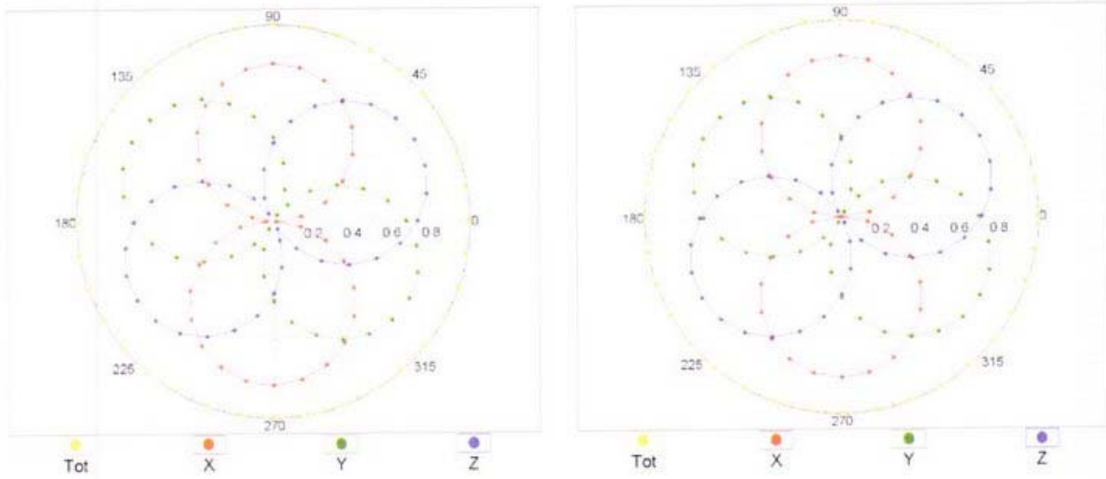
f=600 MHz,TEM
