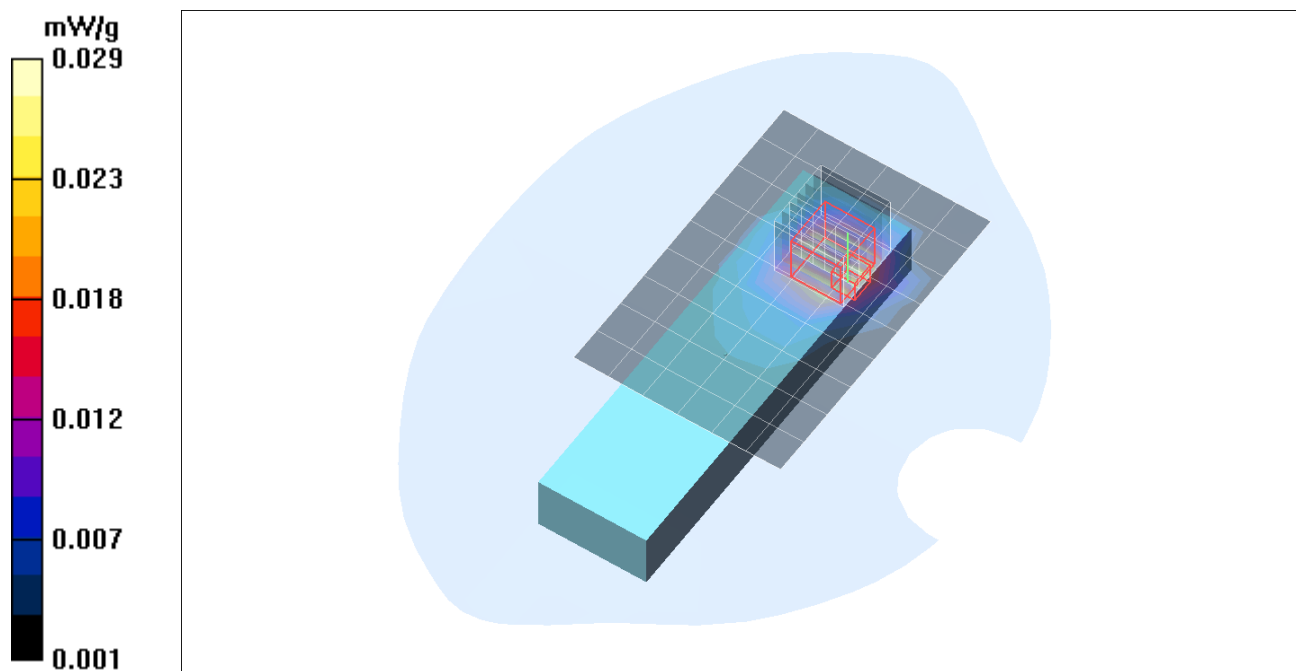
Plot. 2: SAR distribution plot for DECT, channel 0, body-worn configuration, front side, 0mm gap.
