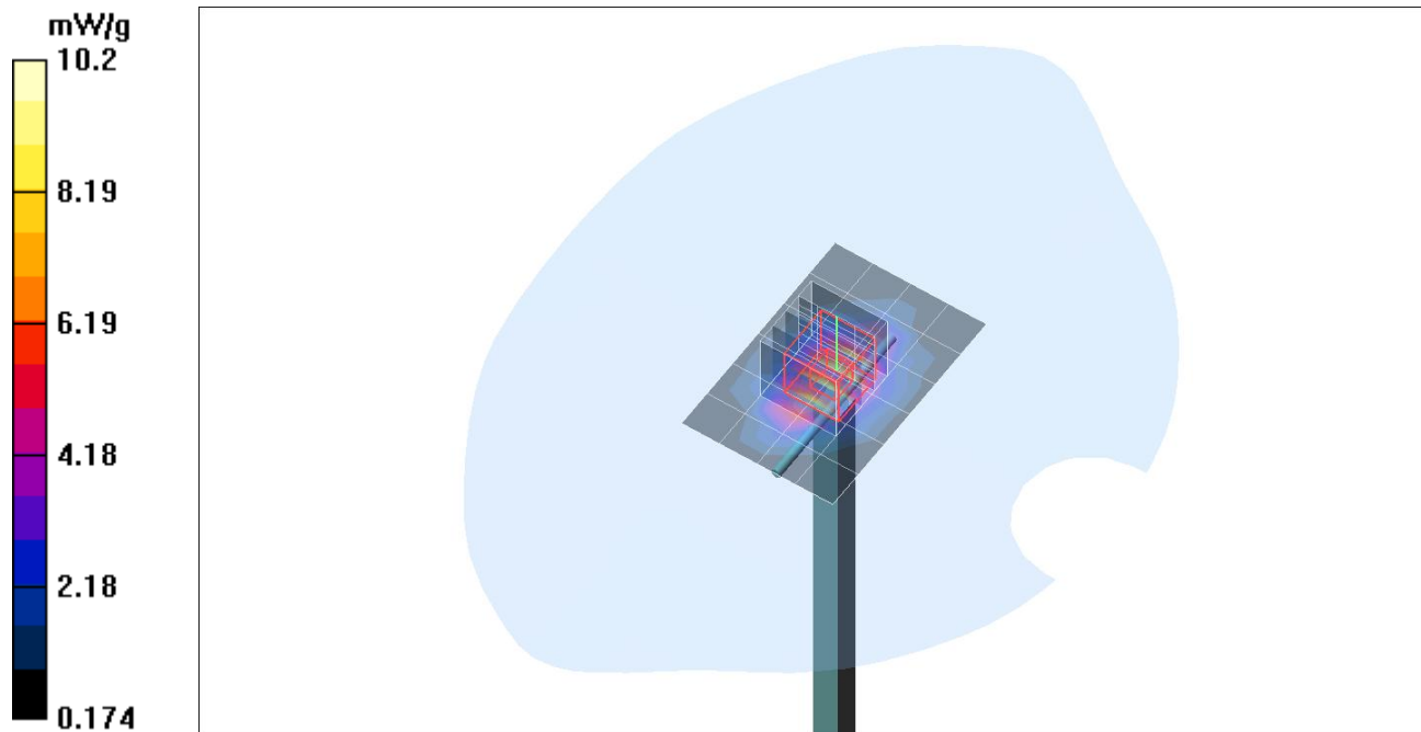
Plot. 3: System Verification Measurement 1900 MHz, Head.
