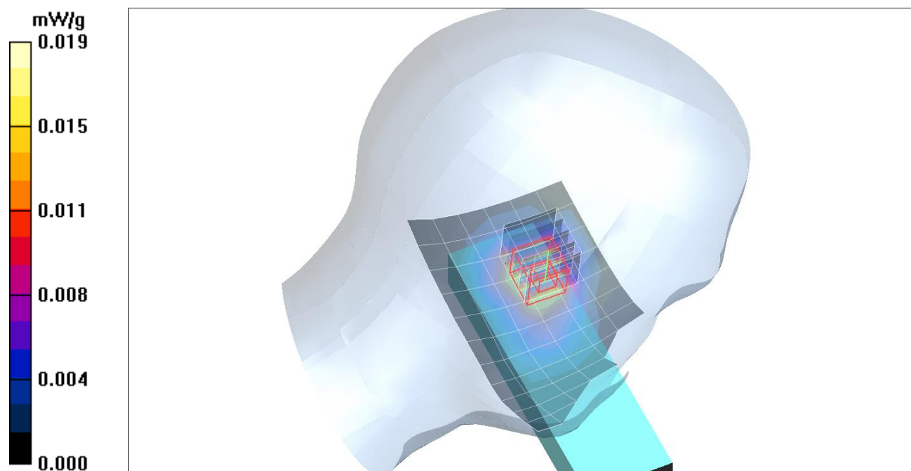
Plot. 1: SAR distribution plot for DECT, channel 0, head configuration, left cheek.
