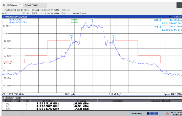
In-Band Unwanted Emissions, Lower Channel
