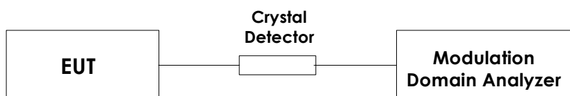
Test Set-up 2
