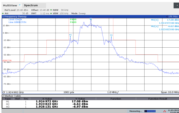
In-Band Unwanted Emissions, Middle Channel
