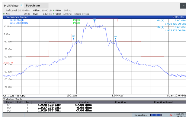
In-Band Unwanted Emissions, Upper Channel
