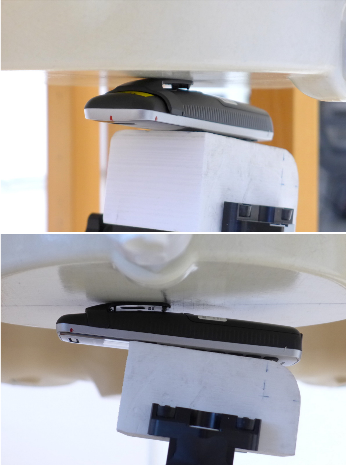
Pic. 8: Test position rear side of DUT towards the phantom, 0 mm gap, belt clip attached.
