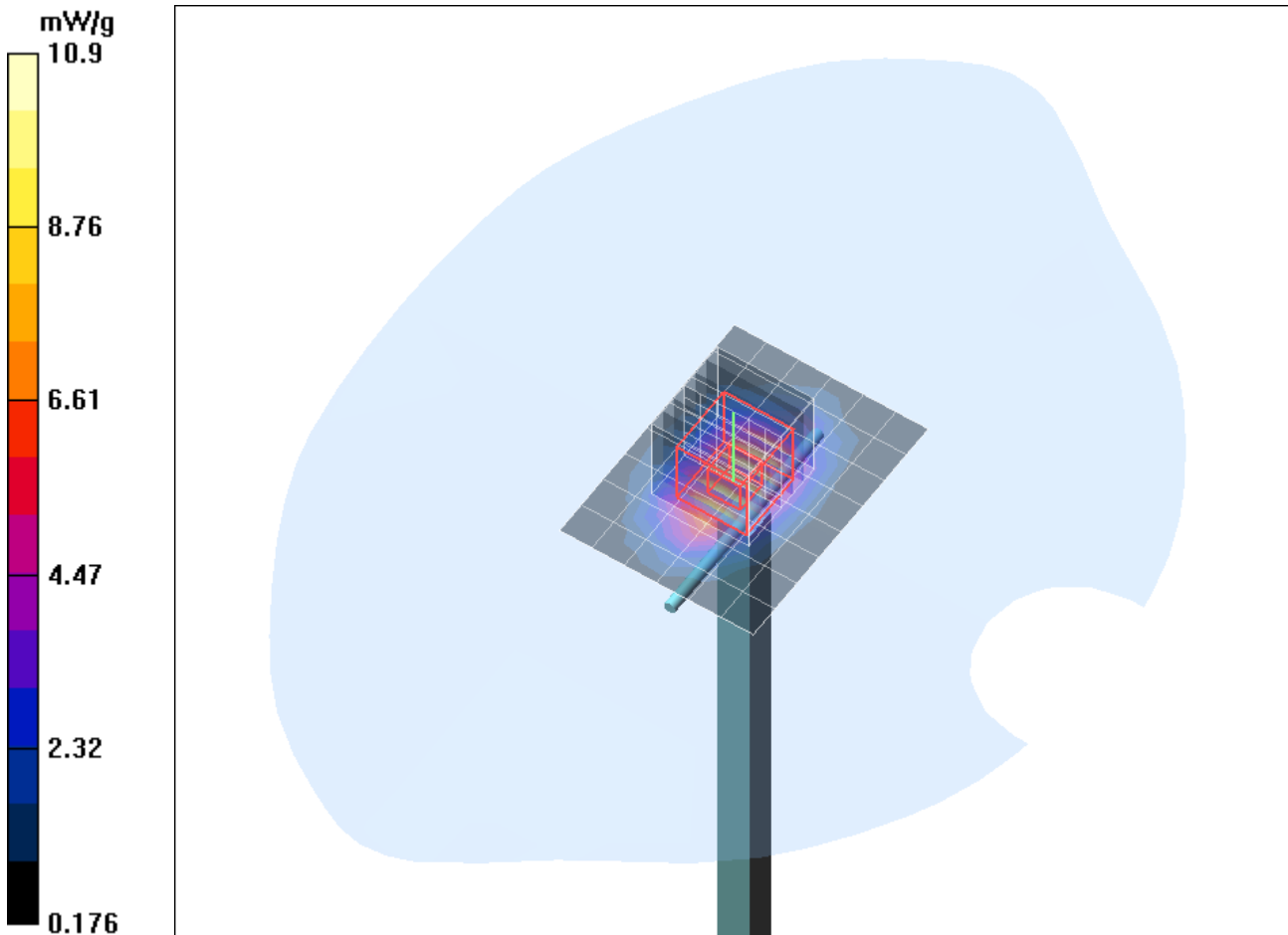
Fig. 8: Validation measurement 1900 MHz Head (November 27, 2014), coarse grid.
