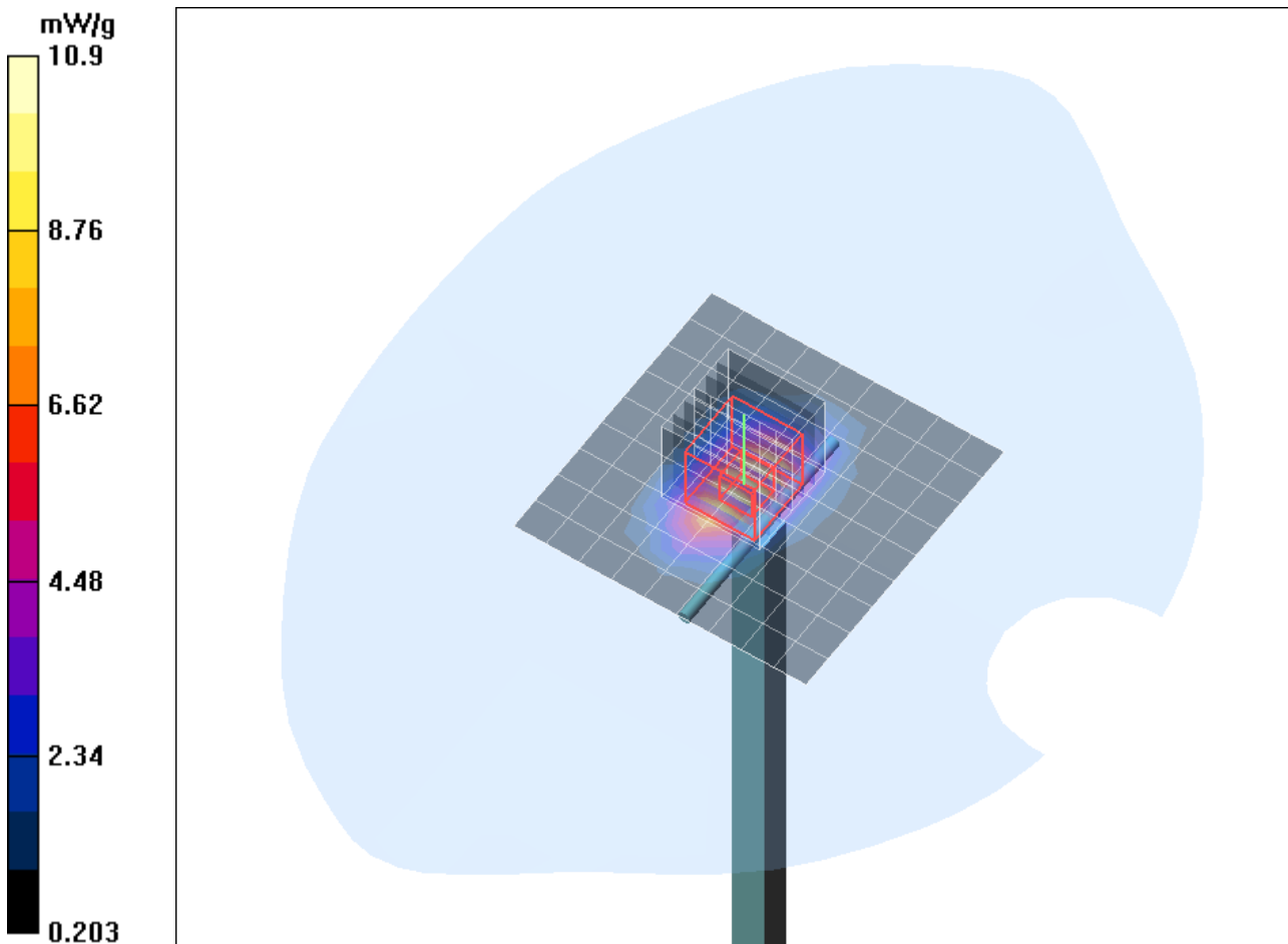
Fig. 9: Validation measurement 1900 MHz Body (December 02, 2014), coarse grid.
