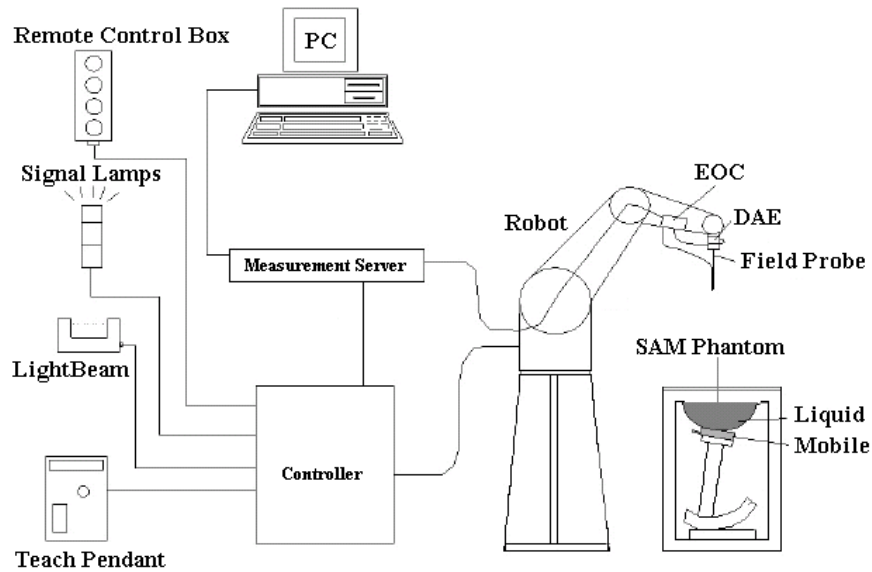
Fig. 7: The DASY4 measurement system.
