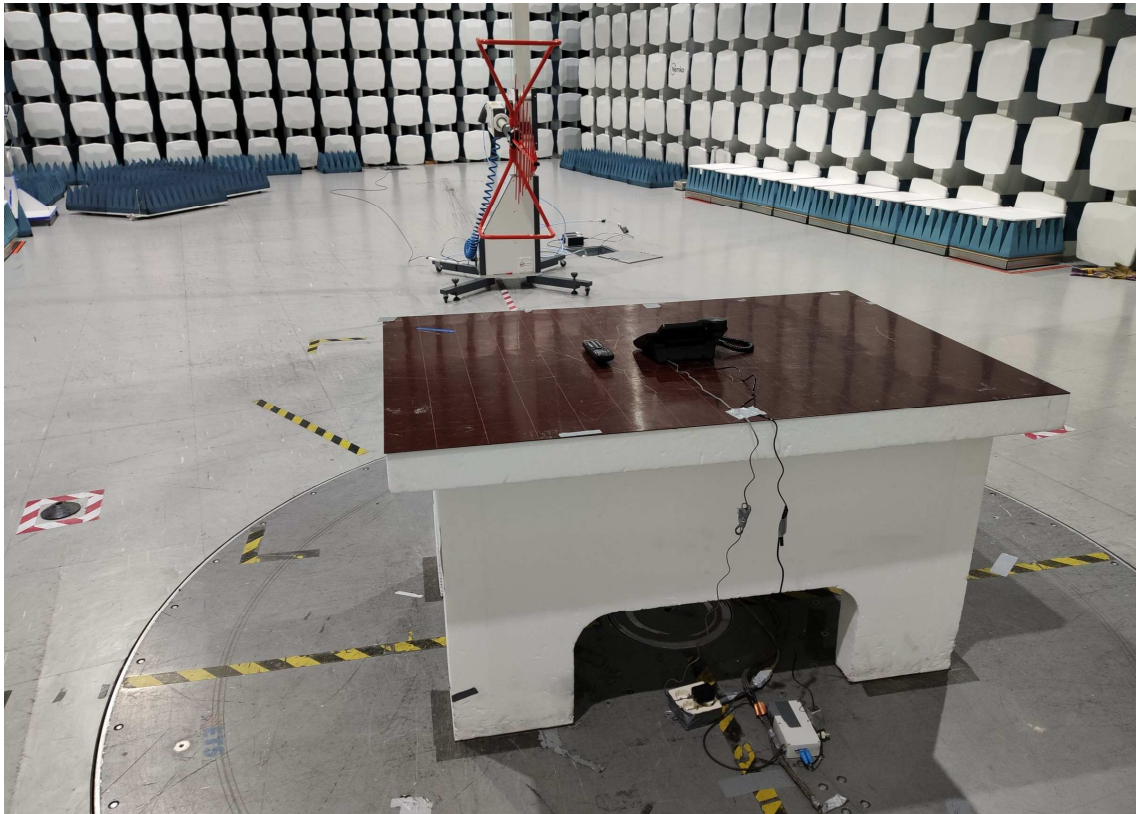
Radiated Emissions, 30 – 1000 MHz
