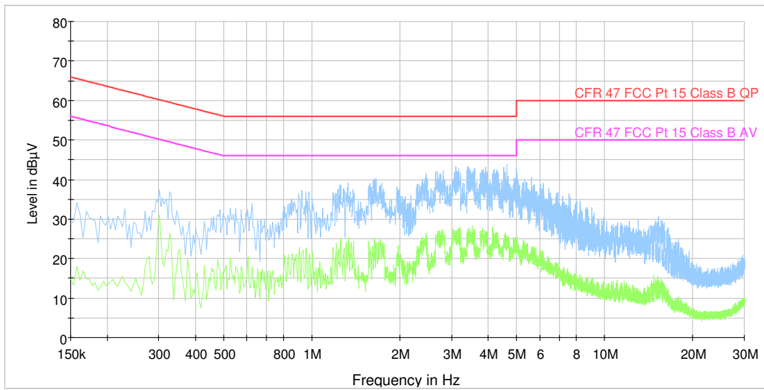
120V 60Hz, ON Hook, handset Charging
