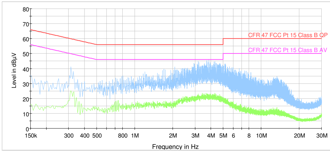
120V 60Hz, OFF Hook
