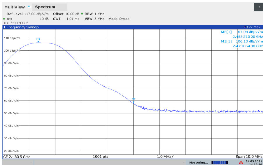
Upper Band Edge 2480 MHz, GFSK, Peak
