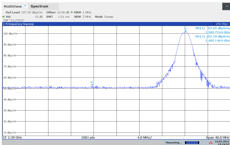
Lower Band Edge 2402 MHz, GFSK, Peak
