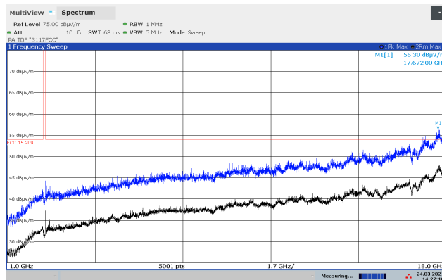
Radiated Emissions 1 - 18 GHz, 2480 MHz, GFSK, VP
