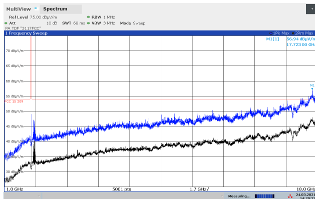
Radiated Emissions 1 - 18 GHz, 2480 MHz, GFSK, HP
