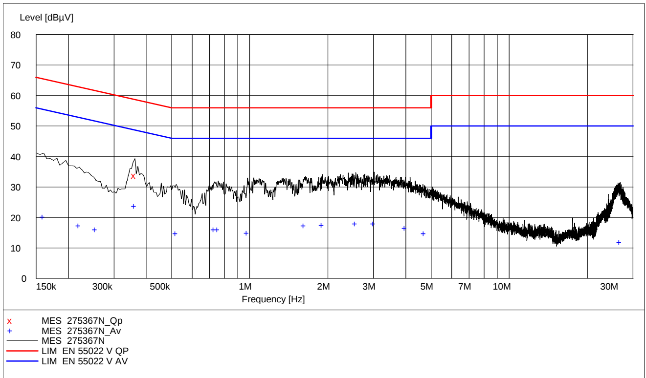
Standby Mode (Plot shows worst case of Phase L1 and N)
