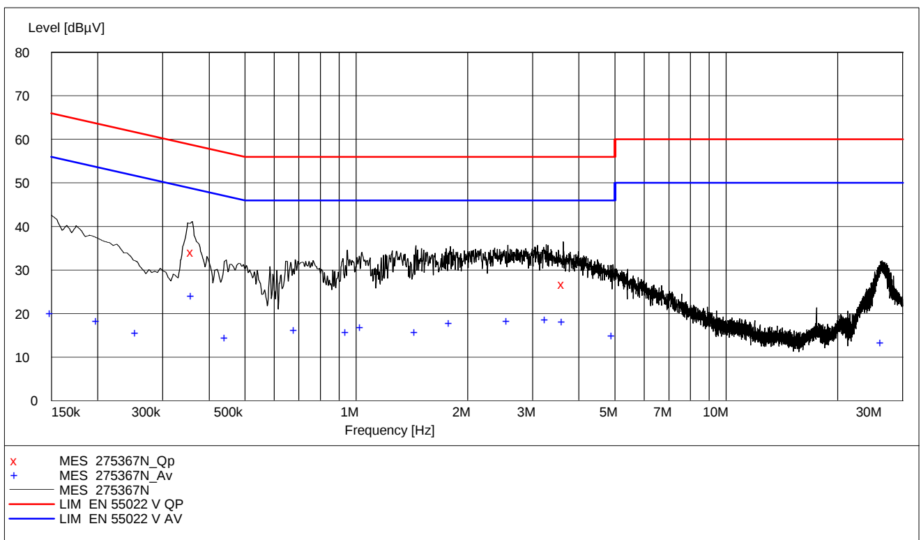
Hook Off Mode (Plot shows worst case of Phase L1 and N)
