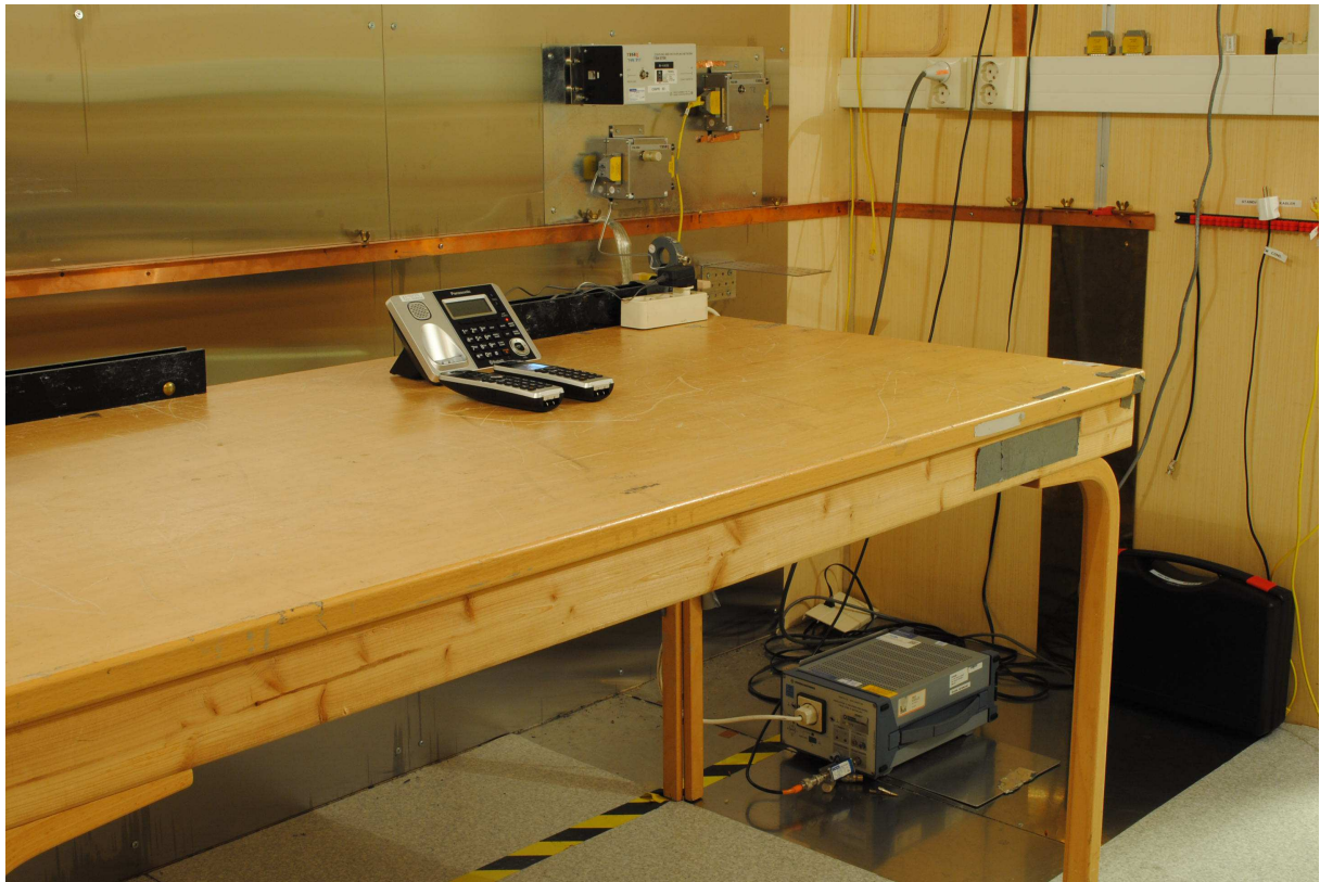
Power line Conducted Emissions Test (Tests were performed on KX-TGF370)
