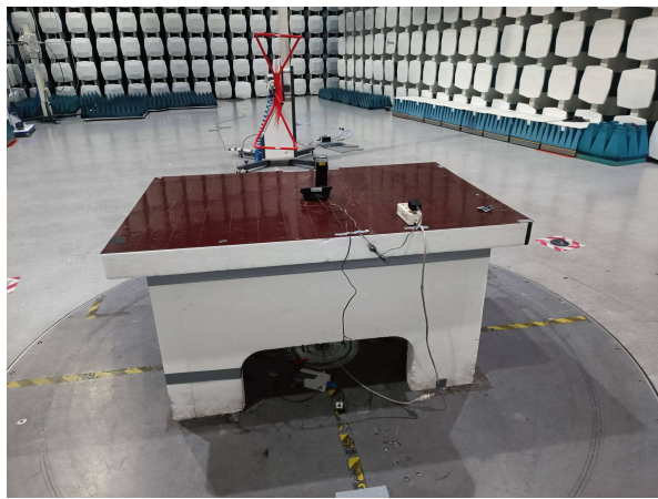
Radiated Emissions
