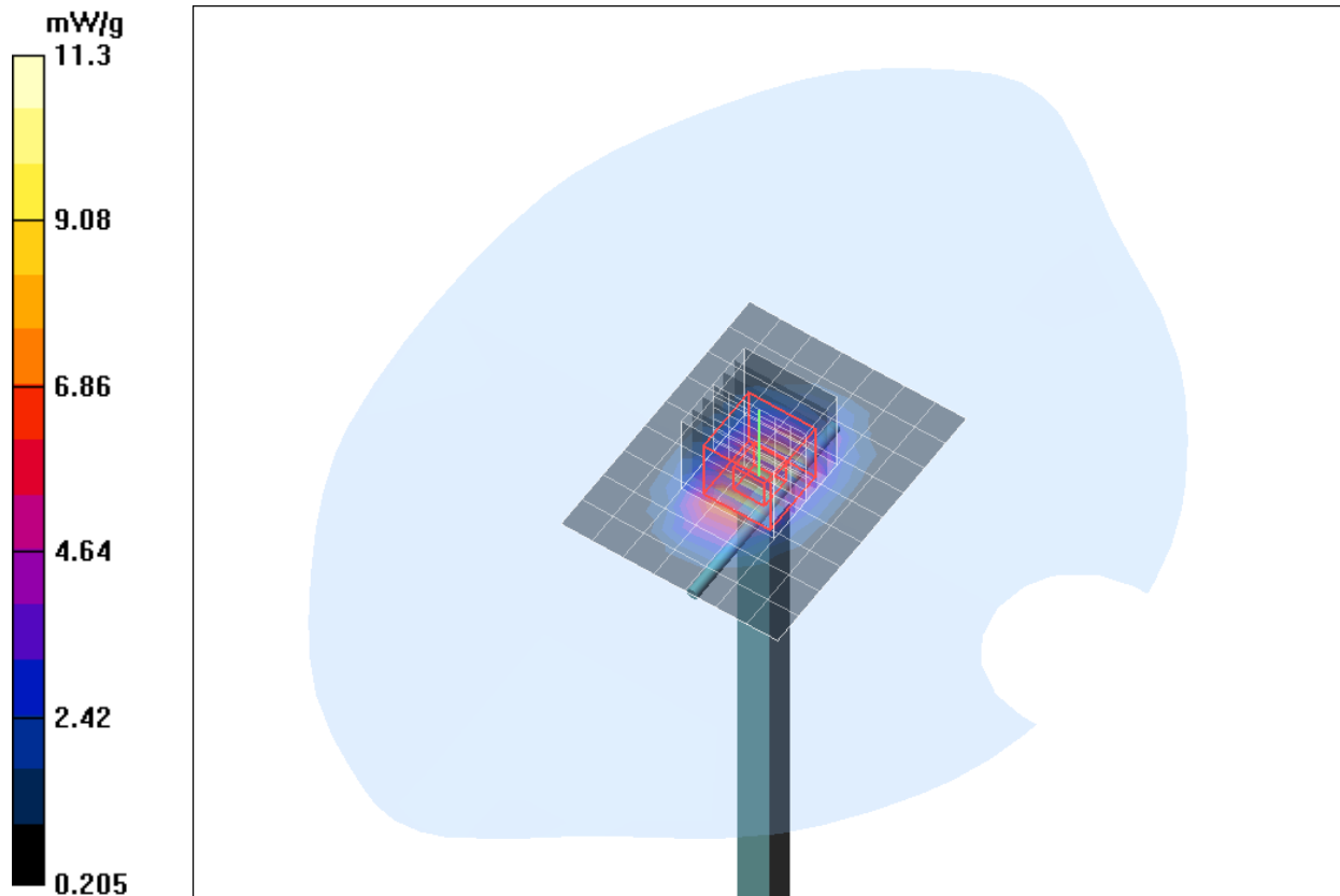
Fig. 8: Validation measurement 1900 MHz Head (July 13, 2015), coarse grid.
