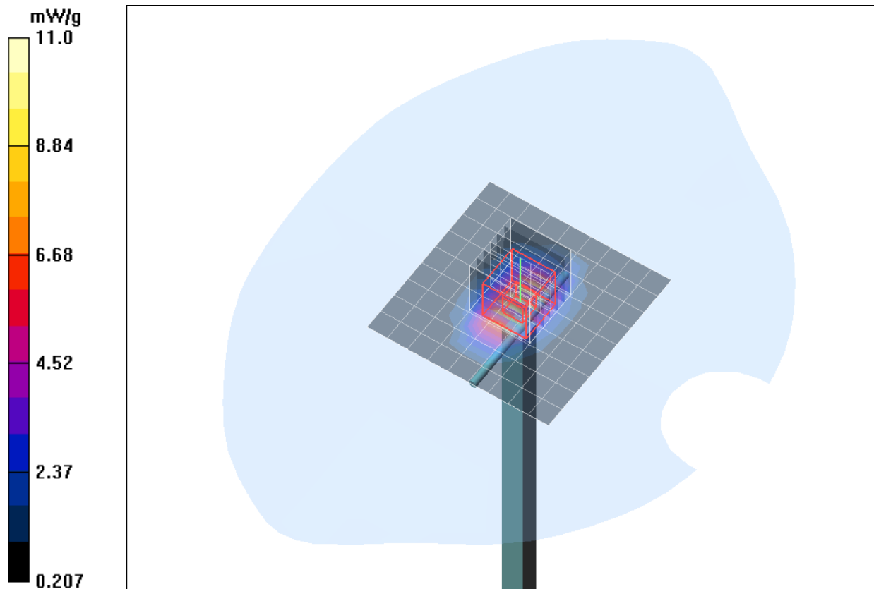
Fig. 9: Validation measurement 1900 MHz Body (July 14, 2015), coarse grid.
