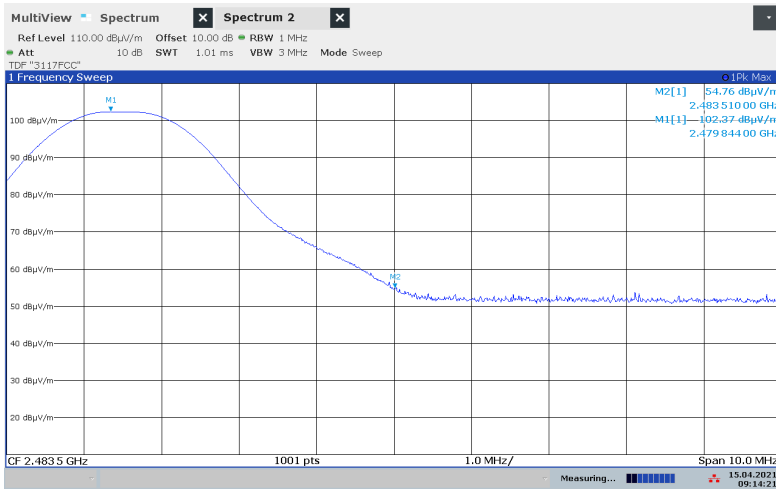
Upper Band Edge 2480 MHz, GFSK, Peak
