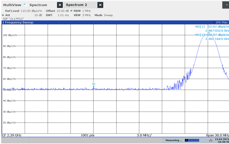
Lower Band Edge 2402 MHz, GFSK, Peak
