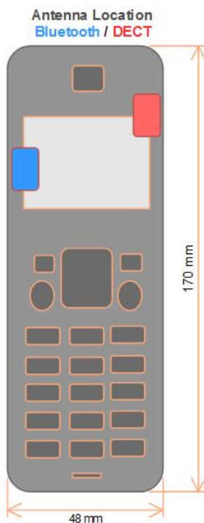
Fig. 1: Sketch of DUT and 1x DECT and 1x BT antenna locations.
