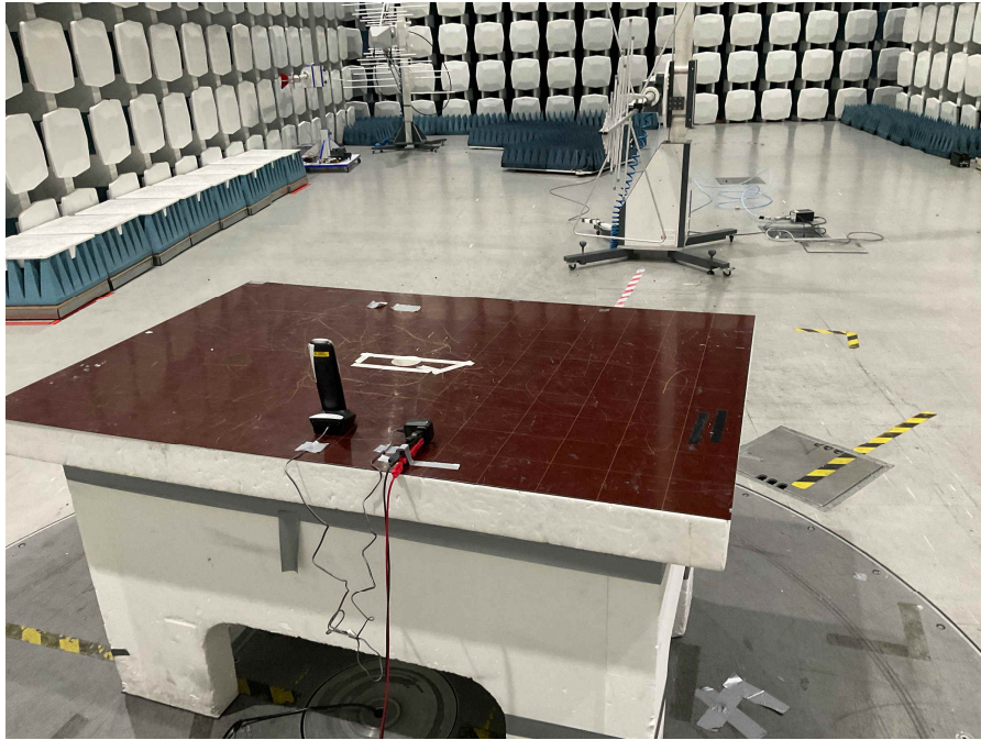
Radiated Emissions 30 – 1000 MHz, Charging
