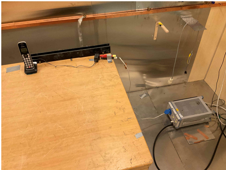
Power-Line Conducted Emissions
