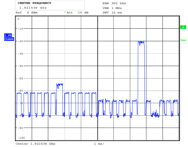
Date: 27.JAN.2022 13:20:52 EUT Transmits on Free RECEIVE Slot, AFTER
