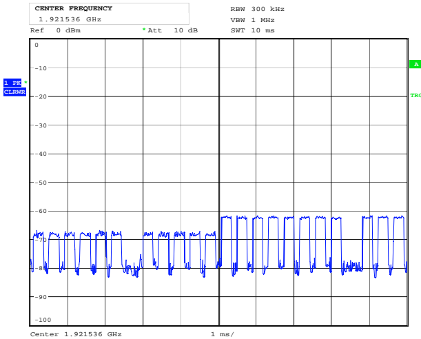
Date: 27.JAN.2022 13:20:07 EUT Transmits on Free TRANSMIT Slot, BEFORE
