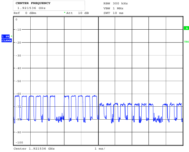
Date: 27.JAN.2022 13:20:39 EUT Transmits on Free RECEIVE Slot, BEFORE
