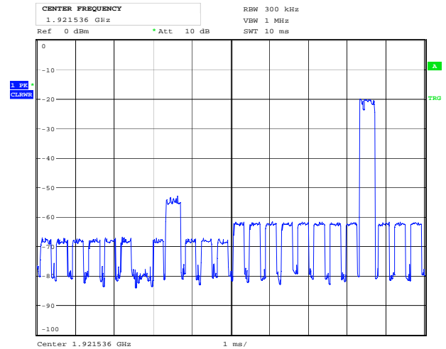
Date: 27.JAN.2022 13:20:18 EUT Transmits on Free TRANSMIT Slot, AFTER
