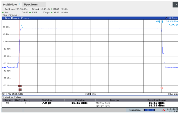
Conducted Peak Output Power, Lower Channel
