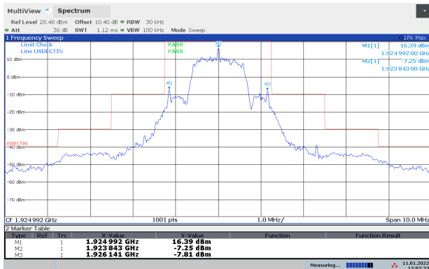
In-Band Unwanted Emissions, Middle Channel
