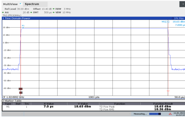
Conducted Peak Output Power, Middle Channel
