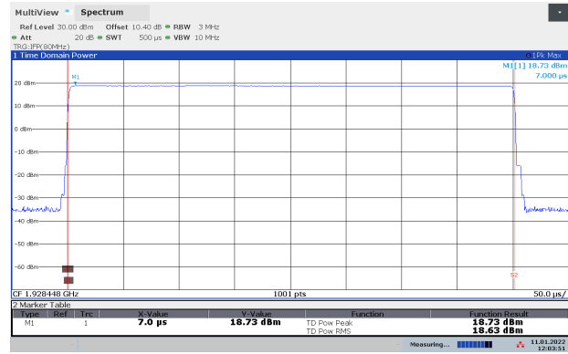
Conducted Peak Output Power, Upper Channel
