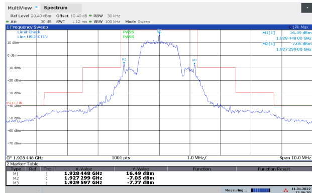
In-Band Unwanted Emissions, Upper Channel
