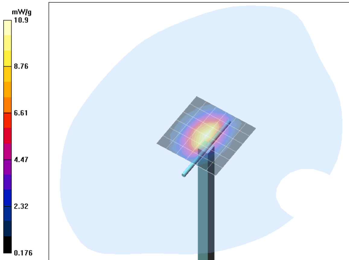
Fig. 10: Validation measurement 1900 MHz Head (May 26, 2008), coarse grid. Ambient Temperature: 21.9° C, Liquid Temperature: 21.1° C.
