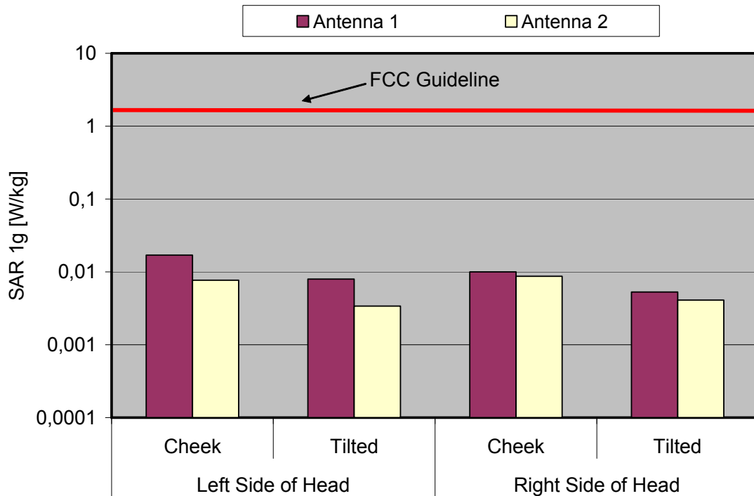
Fig. 8: The measured head phantom SAR values for the Panasonic KX-TGA939 for the US DECT standard in comparison to the FCC exposure limit.
