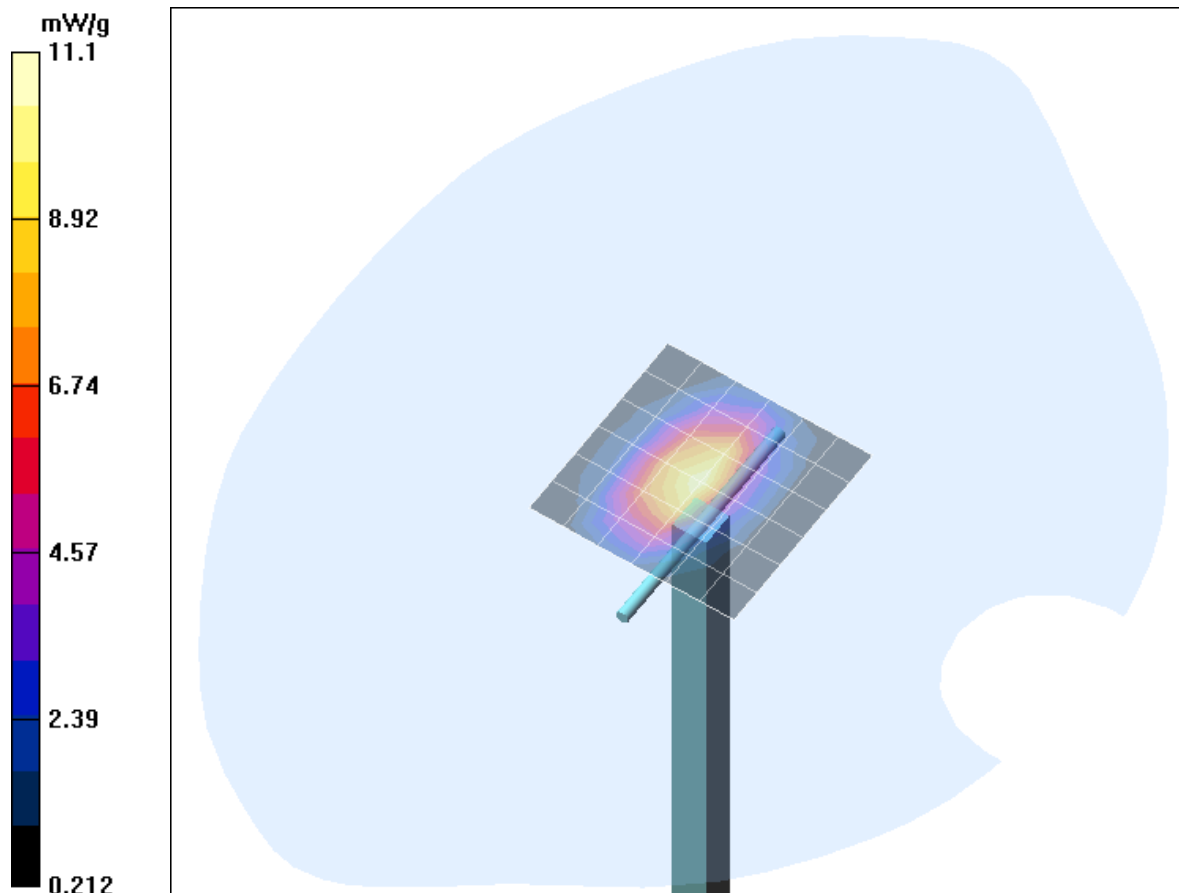
Fig. 11: Validation measurement 1900 MHz body (May 27, 2008), coarse grid. Ambient Temperature: 22.5° C, Liquid Temperature: 21.7° C.
