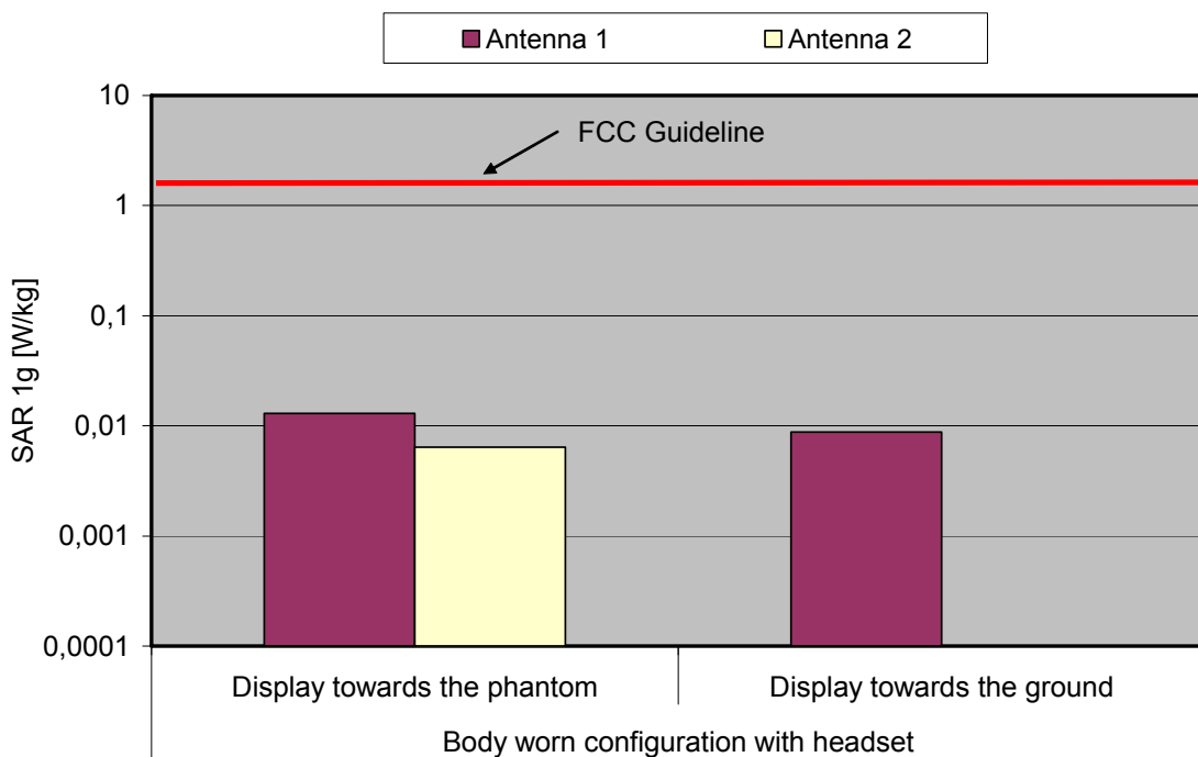
Fig. 9: The measured SAR values in body-worn configuration for the Panasonic KX-TGA939 for the US DECT standard in comparison to the FCC exposure limit.
