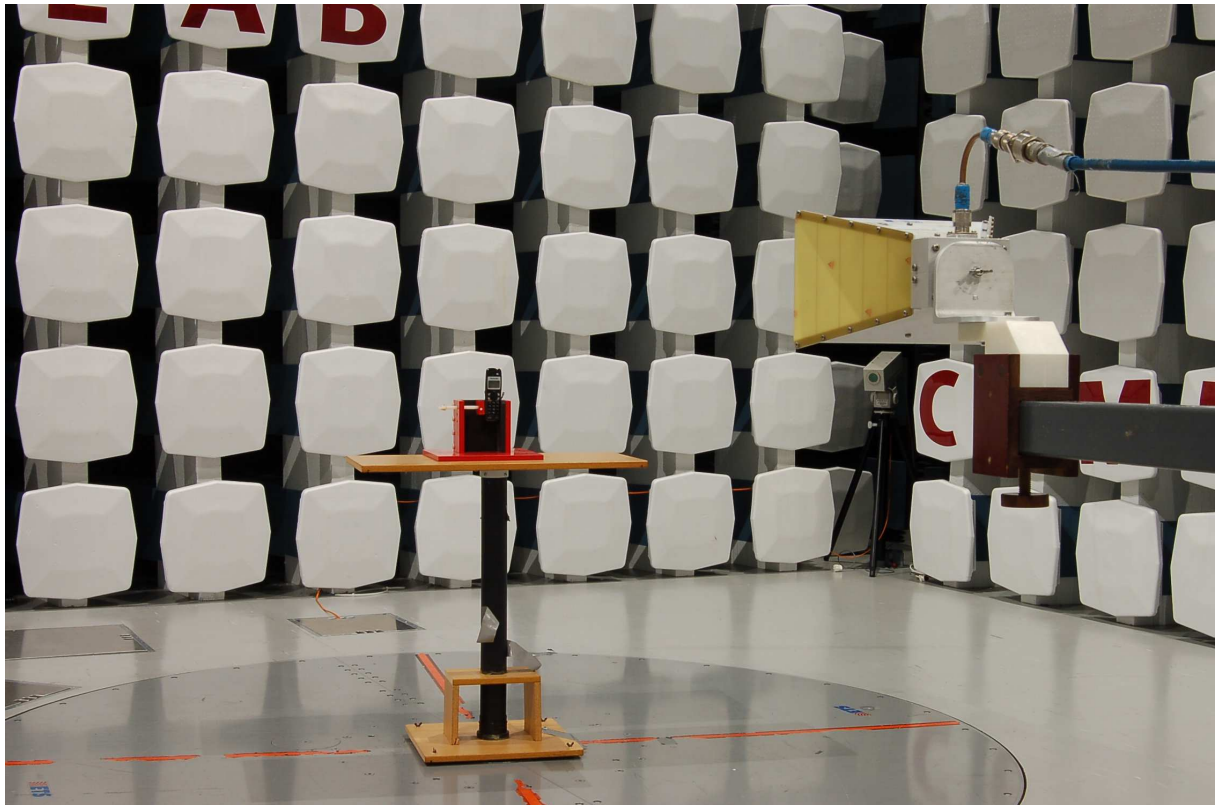
Radiated test - Antenna Gain
