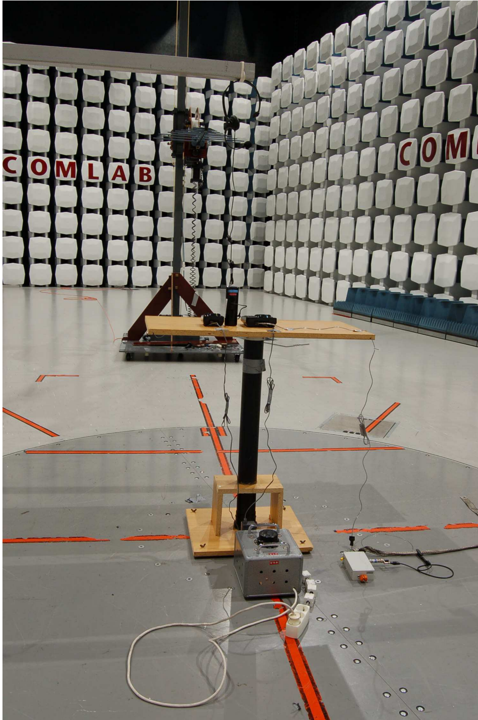
Radiated Emissions Test 200 - 1000 MHz
