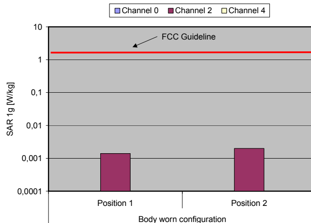
Fig. 9: The measured SAR values in body-worn configuration for the Panasonic KX-TGA820 for the US DECT standard in comparison to the FCC exposure limit.
