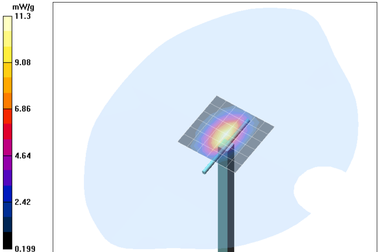
Fig. 11: Validation measurement 1900 MHz body (May 29, 2007), coarse grid. Ambient Temperature: 22.7° C, Liquid Temperature: 21.6° C.
