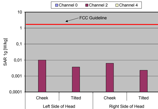
Fig. 8: The measured head phantom SAR values for the Panasonic KX-TGA820 for the US DECT standard in comparison to the FCC exposure limit.
