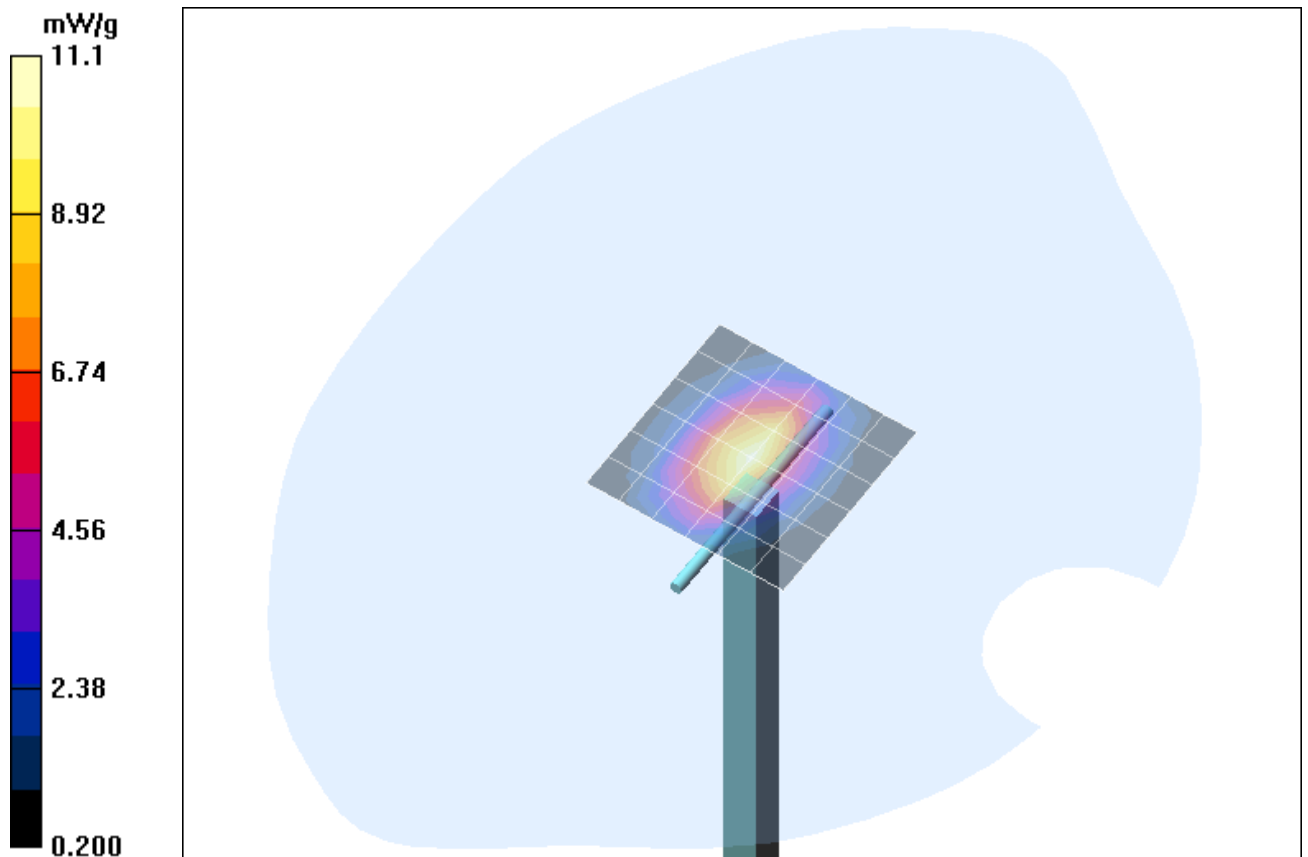
Fig. 10: Validation measurement 1900 MHz Head (May 30, 2007), coarse grid. Ambient Temperature: 22.4° C, Liquid Temperature: 21.3° C.
