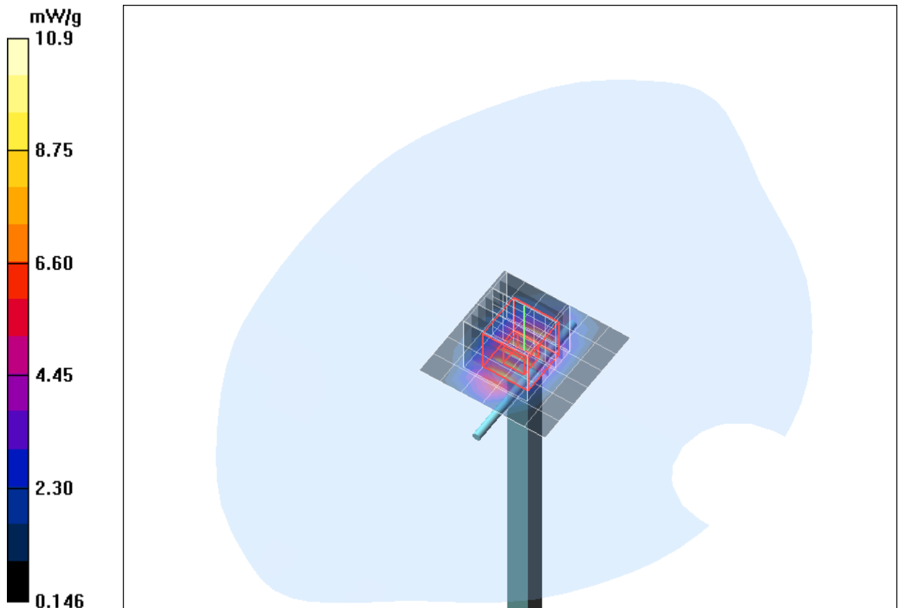
Fig. 11: Validation measurement 1900 MHz body (November 29, 2010), coarse grid. Ambient Temperature: 21.4° C, Liquid Temperature: 21.2° C.
