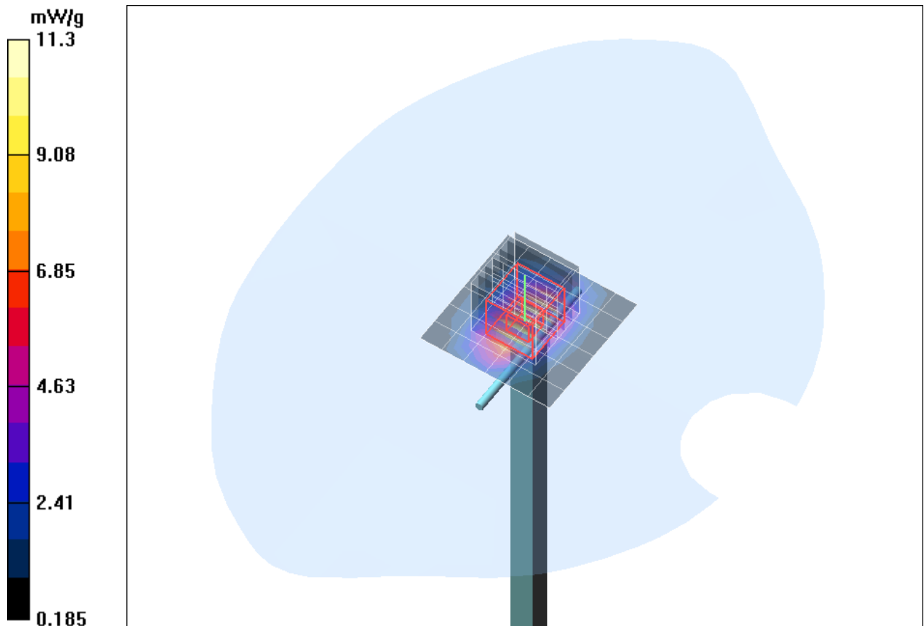
Fig. 10: Validation measurement 1900 MHz Head (November 24, 2010), coarse grid. Ambient Temperature: 20.9° C, Liquid Temperature: 20.6° C.
