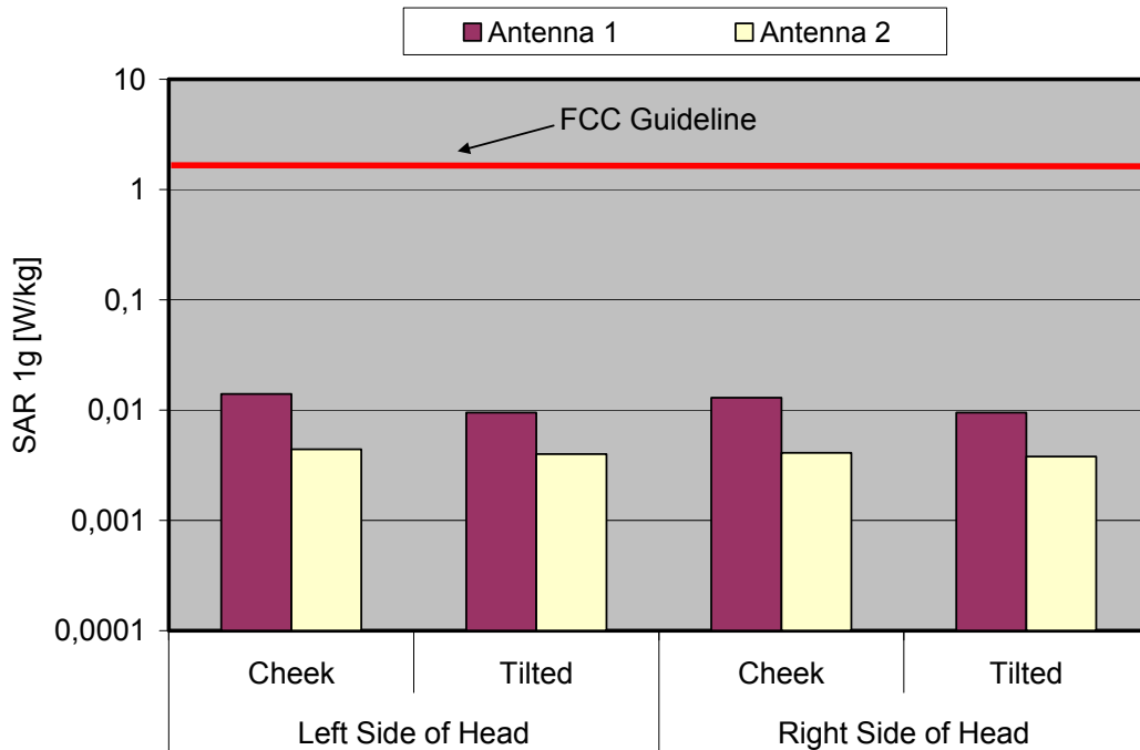
Fig. 8: The measured head phantom SAR values for the Panasonic KX-TGA740 for the US DECT standard in comparison to the FCC exposure limit.
