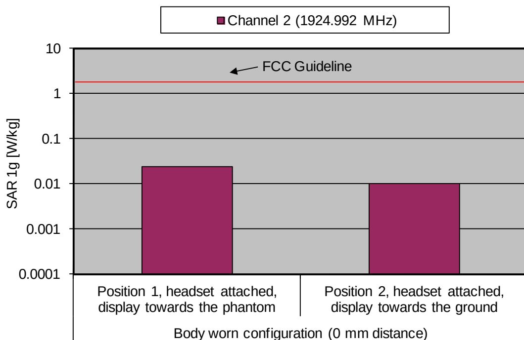
Fig. 9: The measured SAR values in body worn configuration for the Panasonic KX-TGA470 for the US DECT standard in comparison to the FCC exposure limit.
