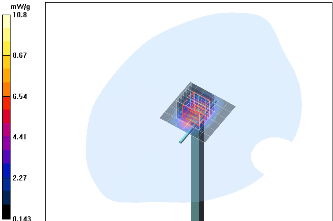
Fig. 11: Validation measurement 1900 MHz body (November 23, 2011), coarse grid. Ambient Temperature: 21.3° C, Liquid Temperature: 20.9° C.
