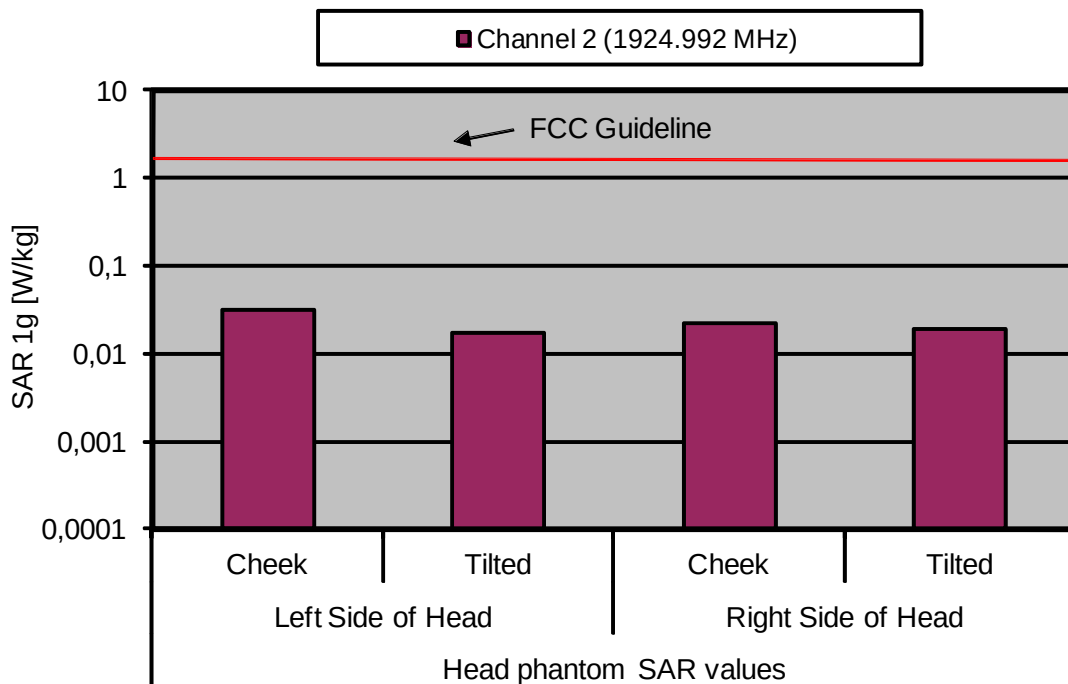
Fig. 8: The measured head phantom SAR values for the Panasonic KX-TGA470 for the US DECT standard in comparison to the FCC exposure limit.
