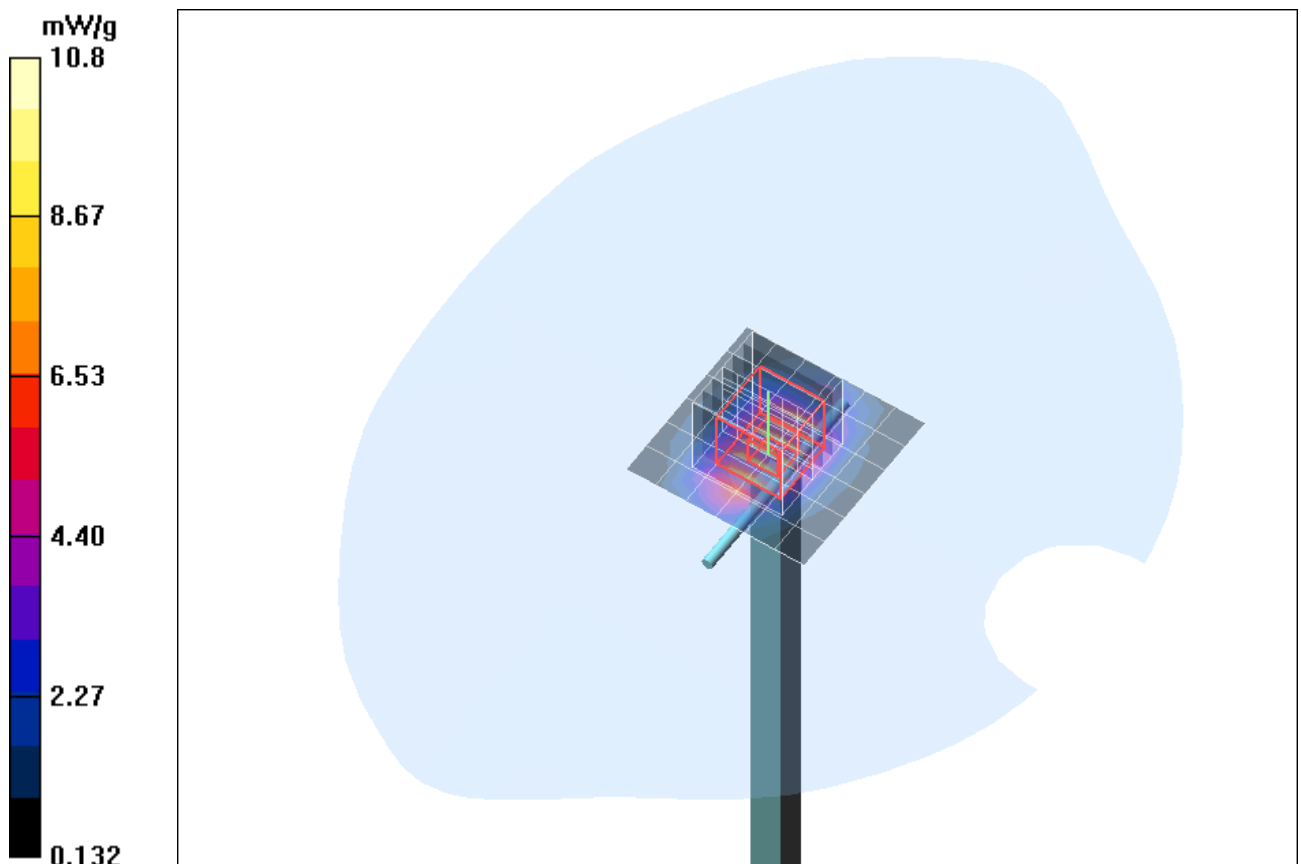
Fig. 10: Validation measurement 1900 MHz Head (November 16, 2011), coarse grid. Ambient Temperature: 21.7° C, Liquid Temperature: 21.3° C.
