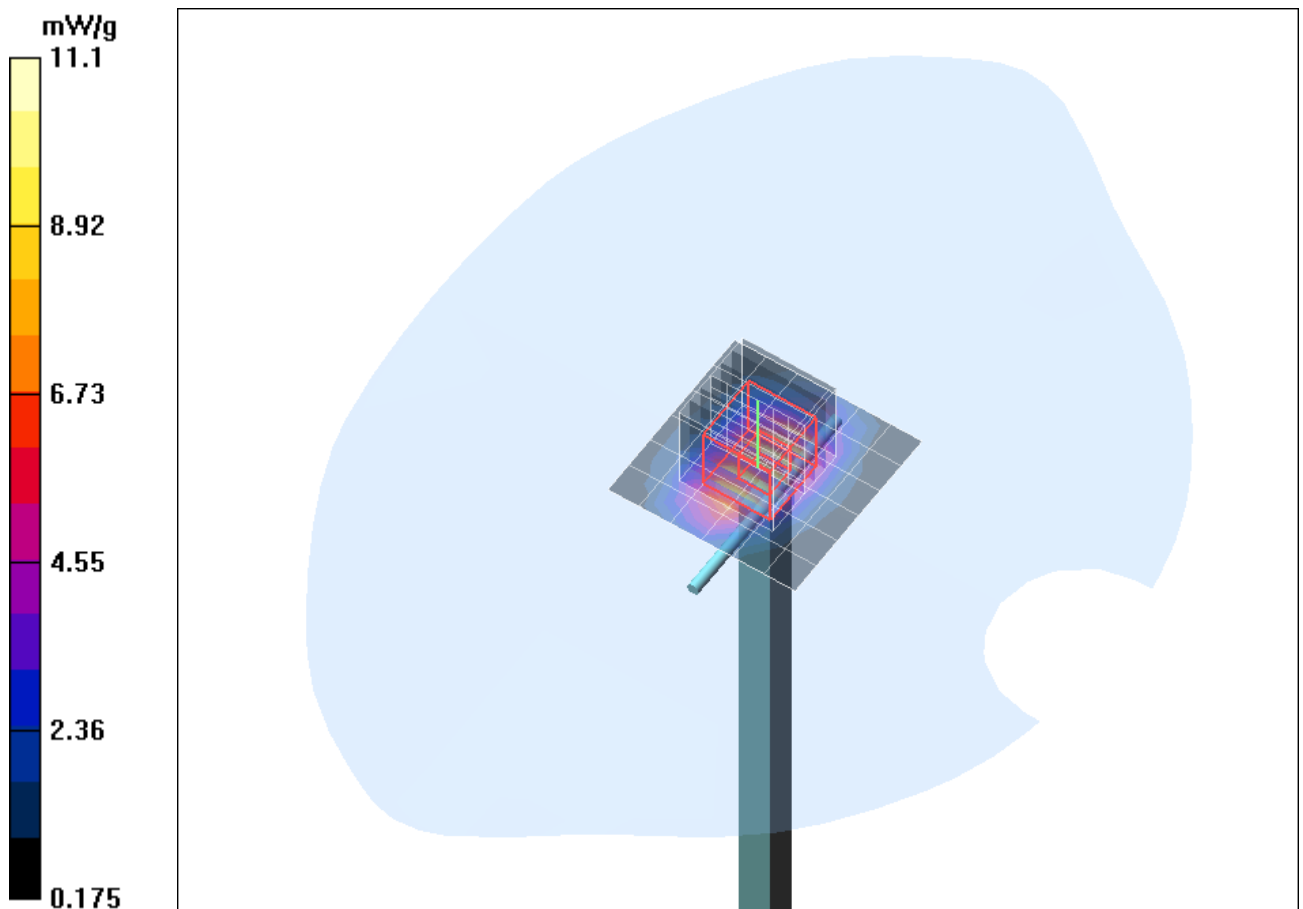
Fig. 9: Validation measurement 1900 MHz Head (March 20, 2012), coarse grid. Ambient Temperature: 22.3° C, Liquid Temperature: 22.1° C.
