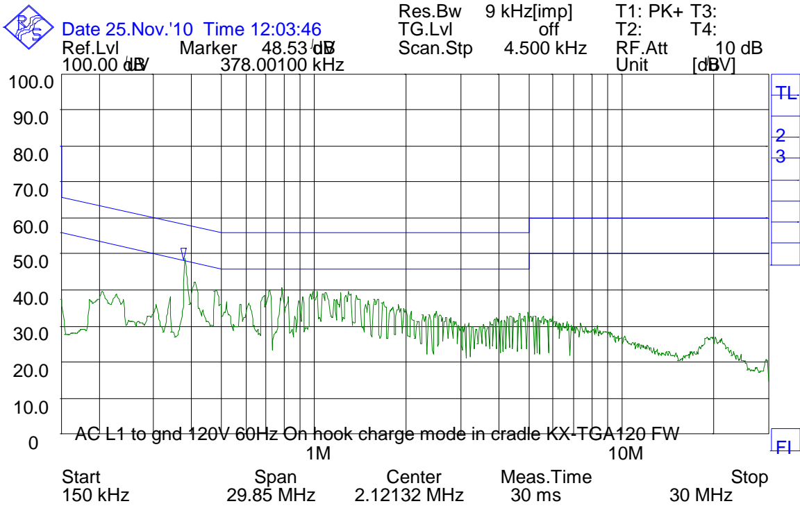
Phase L1, Hook On, Charging, PNLV226(FW)
