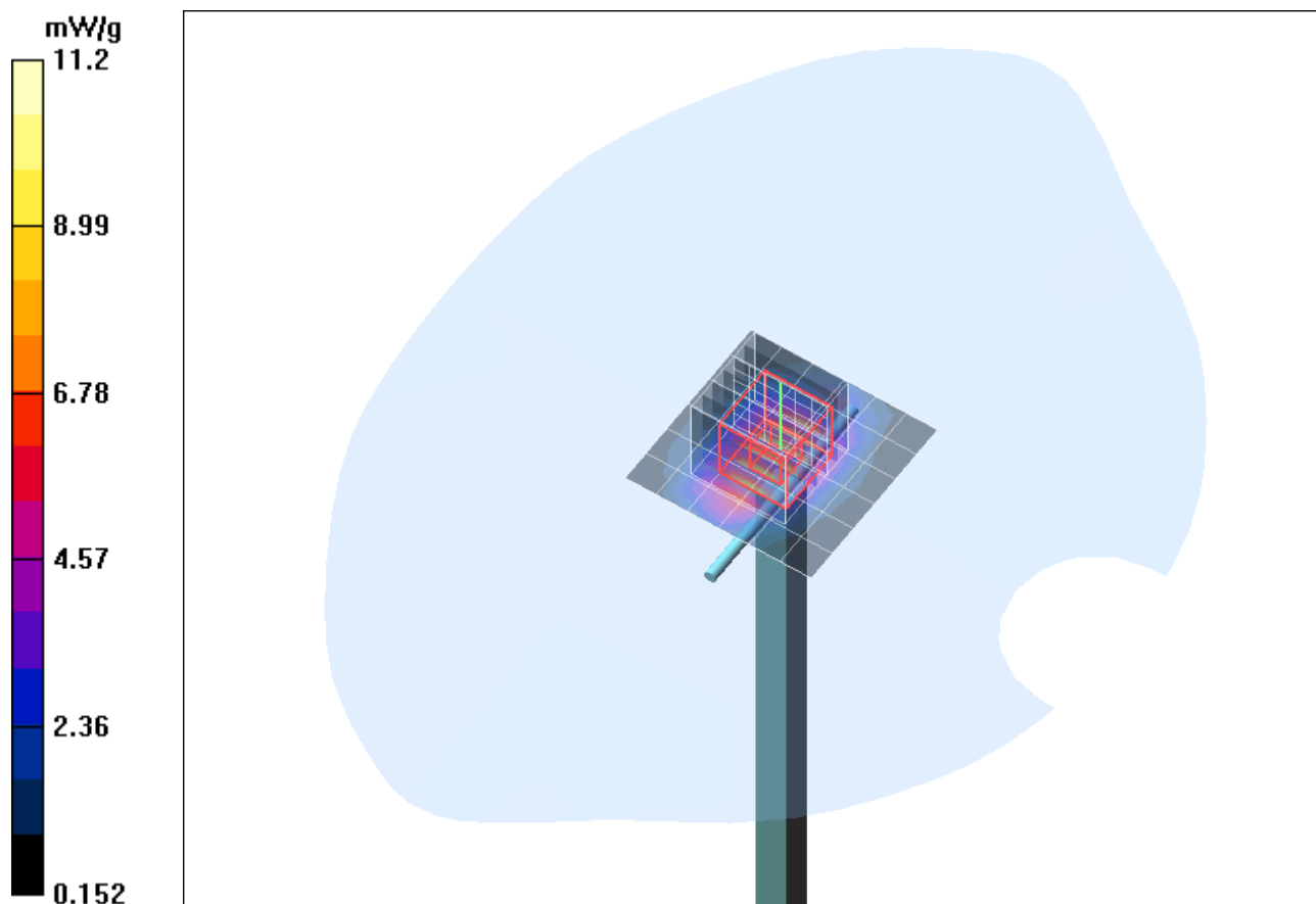
Fig. 9: Validation measurement 1900 MHz Head (November 25, 2010), coarse grid. Ambient Temperature: 21.3° C, Liquid Temperature: 21.0° C.
