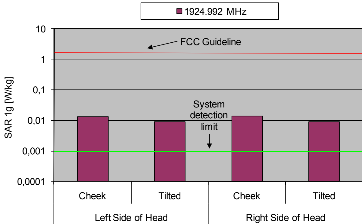
Fig. 8: The measured head phantom SAR values for the Panasonic KX-TGA120 for the US DECT standard in comparison to the FCC exposure limit.
