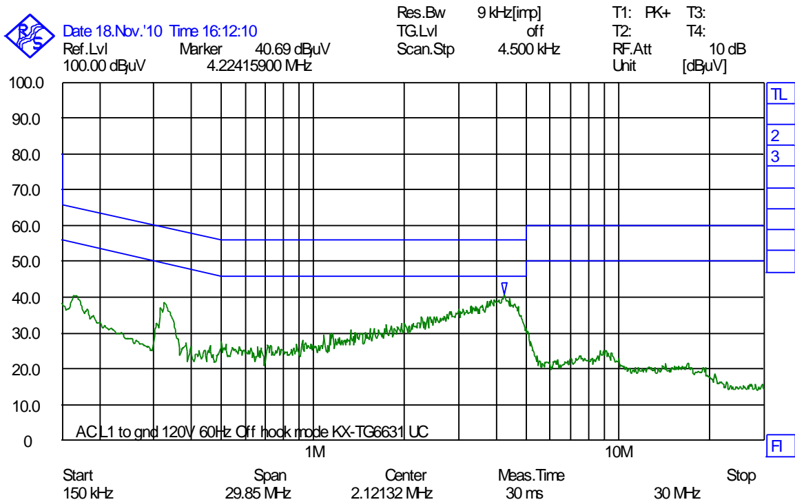
Phase L1, Hook Off, AC Adaptor PNLV226(UC)
