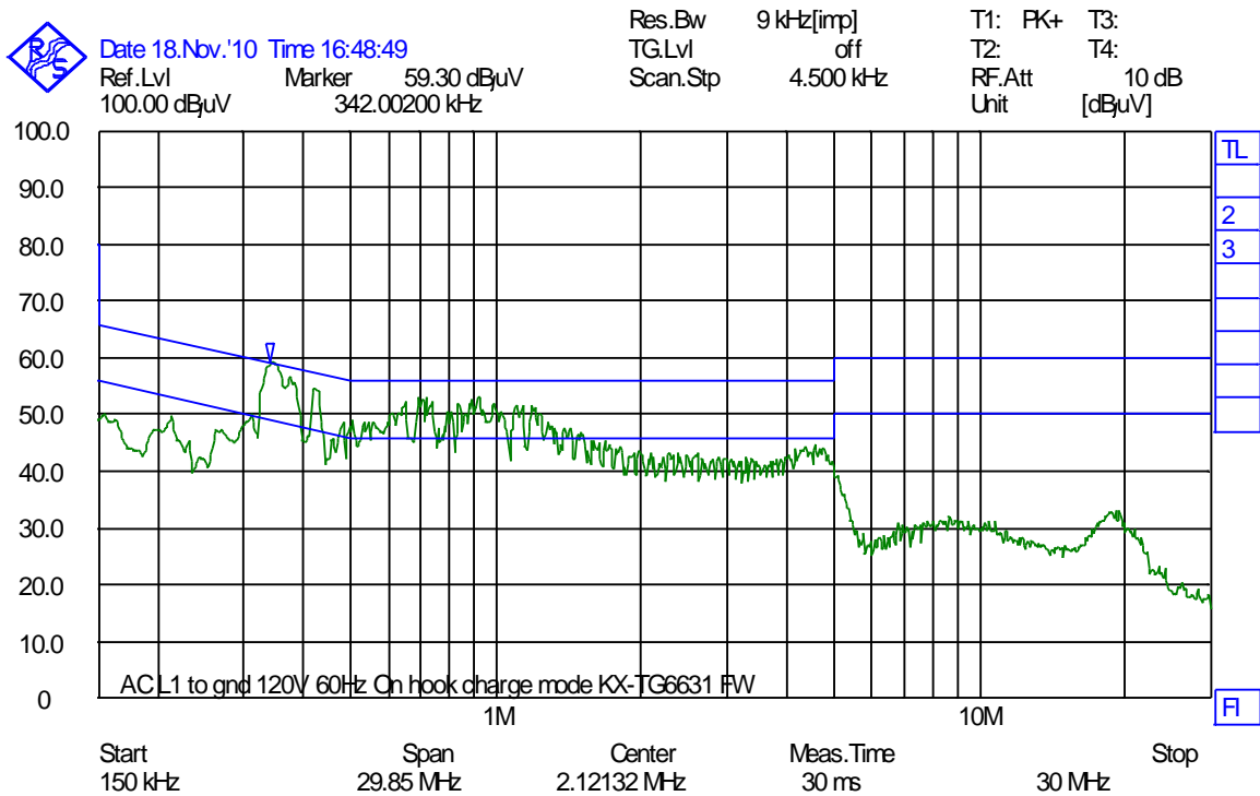
Phase L1, Hook On, Charge Mode, AC Adaptor PNLV226(FW)
