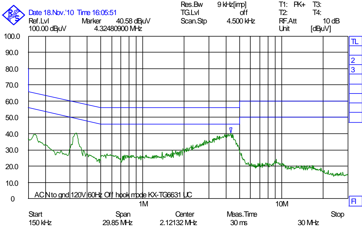
Phase N, Hook Off, AC Adaptor PNLV226(UC)
