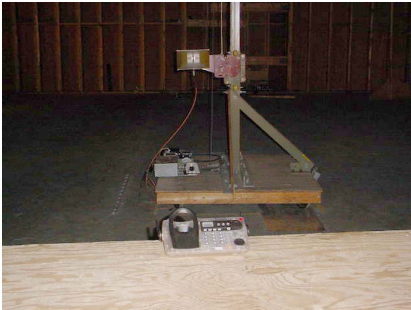
Transmitter Radiated Emissions at 3 Meters Base Unit (Antenna parallel to ground plane)
