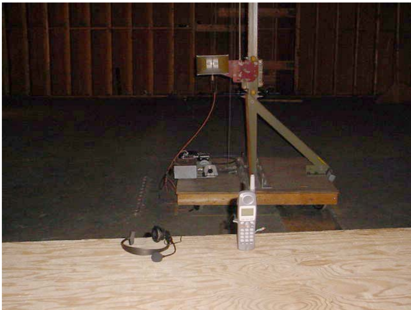
Transmitter Radiated Emissions at 3 Meters Handset (Orthogonal Position # 3)
