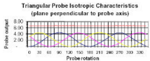
Figure 3.3 Sample Probe Characteristics
