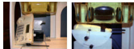
Figure 14.1 Body SAR Test Setup --Base and Hand Set--
