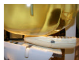
Figure 14.3 Head SAR Test Setup -- Right-Touch --
