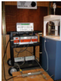
Figure 12.1 Dipole Validation Test Setup
