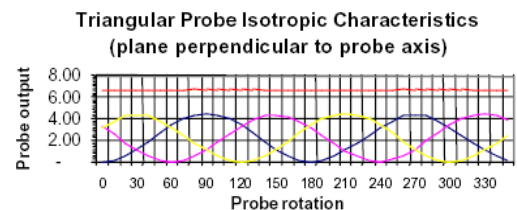
Figure 3.3 Sample Probe Characteristics
