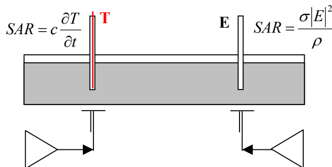
4.1 Temperature Assessment Test Configuration at 5.8 GHz
